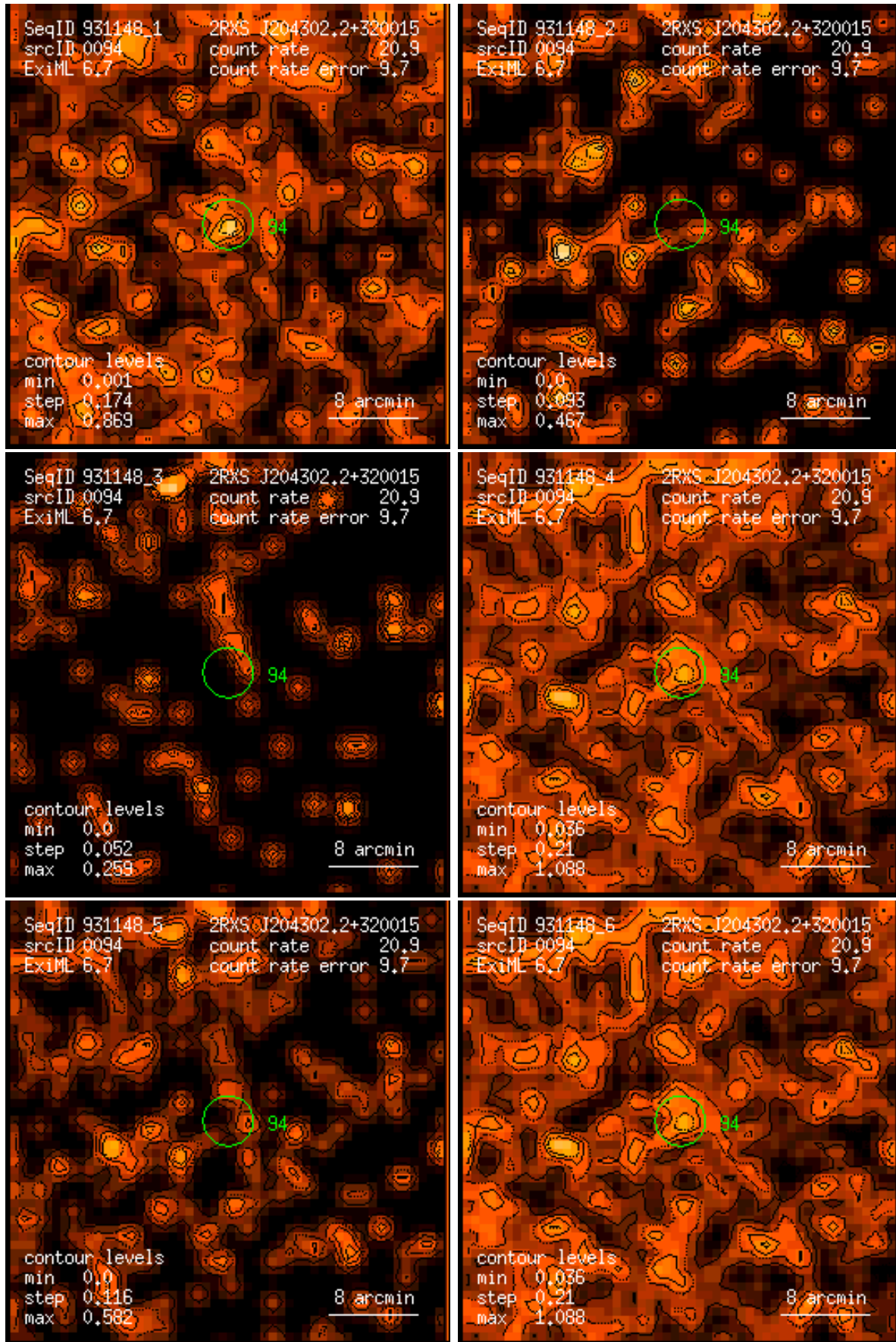
Figure 94: RASS 931148: detection 0094: band rate images, Gaussian filter: (1) PSPC channels 11 – 41, (2) 52 – 90, (3) 91 – 201, (4) 11 – 235, (5) 52 – 201, (6) 11 – 201. Broad band rates in counts/ks. Band rate contour levels in counts/ks/arcmin 2 .
