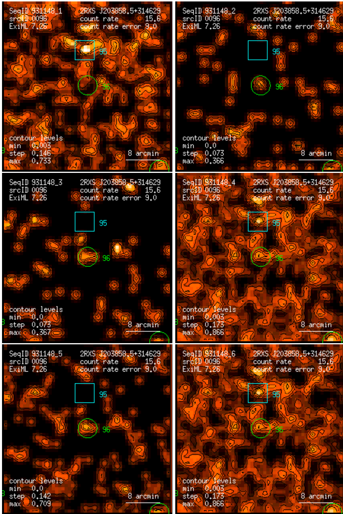
Figure 96: RASS 931148: detection 0096: band rate images, Gaussian filter: (1) PSPC channels 11 – 41, (2) 52 – 90, (3) 91 – 201, (4) 11 – 235, (5) 52 – 201, (6) 11 – 201. Broad band rates in counts/ks. Band rate contour levels in counts/ks/arcmin 2 .
