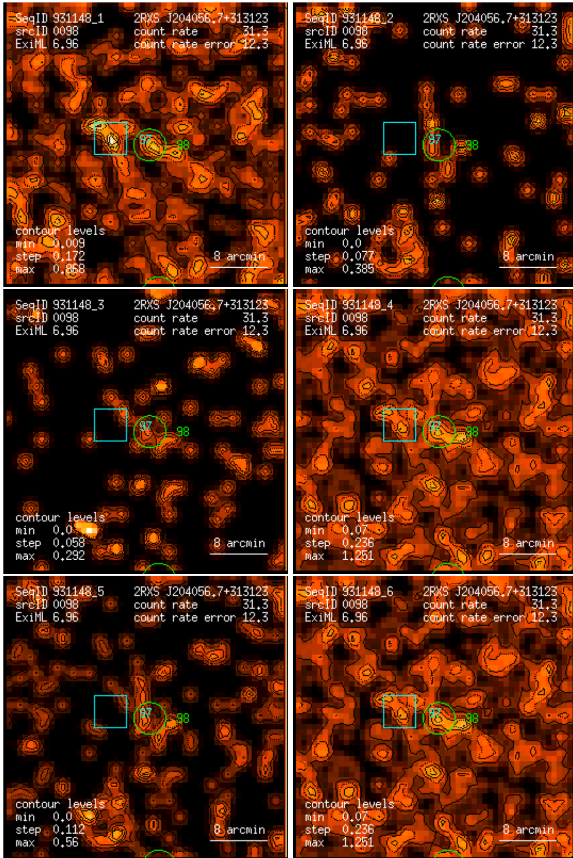
Figure 98: RASS 931148: detection 0098: band rate images, Gaussian filter: (1) PSPC channels 11 – 41, (2) 52 – 90, (3) 91 – 201, (4) 11 – 235, (5) 52 – 201, (6) 11 – 201. Broad band rates in counts/ks. Band rate contour levels in counts/ks/arcmin 2 .
