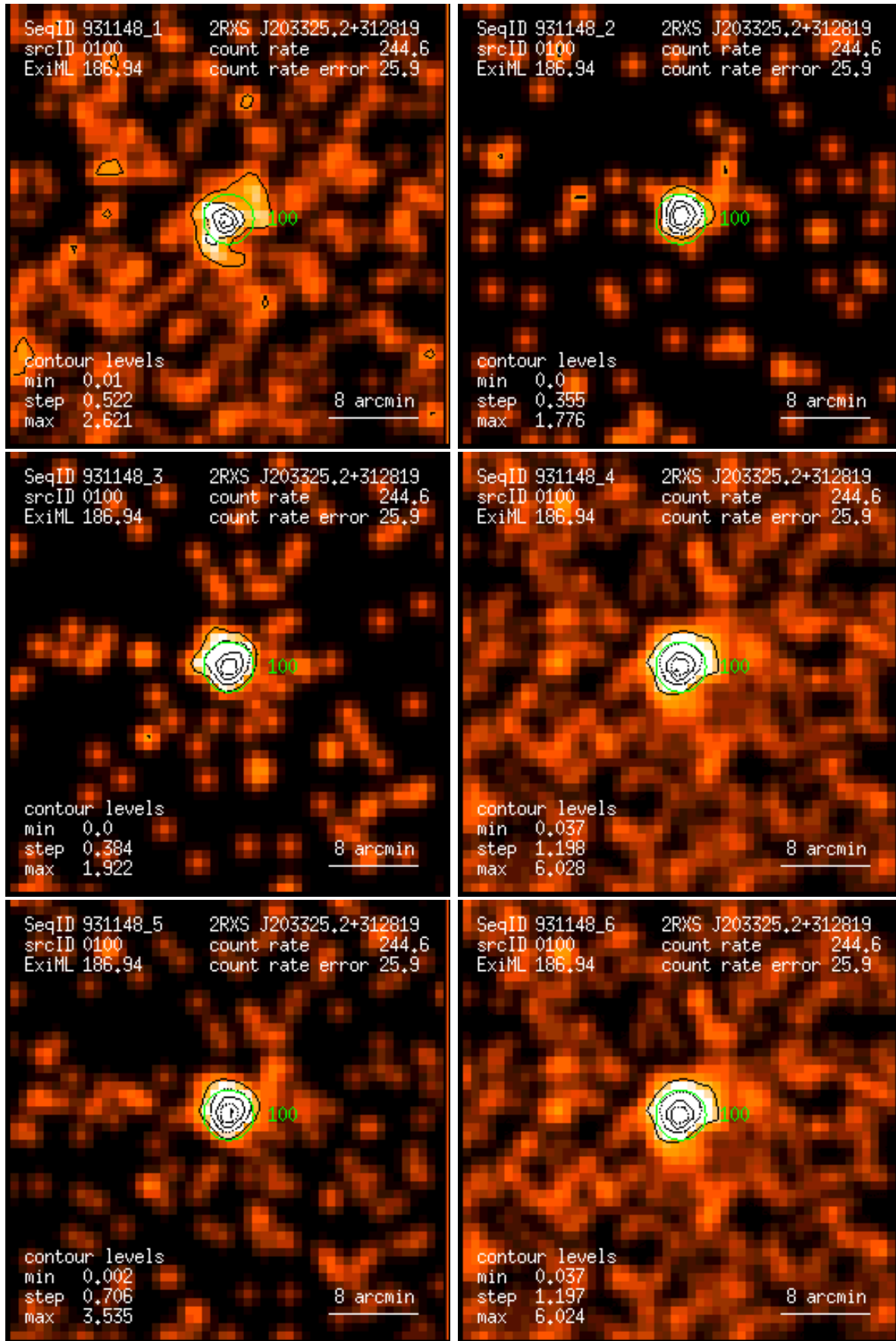
Figure 100: RASS 931148: detection 0100: band rate images, Gaussian filter: (1) PSPC channels 11 – 41, (2) 52 – 90, (3) 91 – 201, (4) 11 – 235, (5) 52 – 201, (6) 11 – 201. Broad band rates in counts/ks. Band rate contour levels in counts/ks/arcmin 2 .
