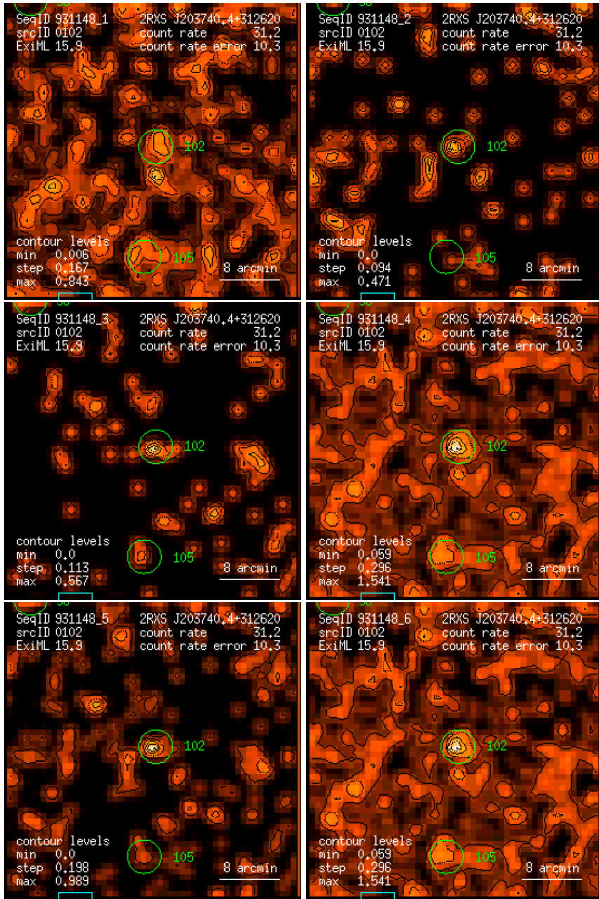
Figure 102: RASS 931148: detection 0102: band rate images, Gaussian filter: (1) PSPC channels 11 – 41, (2) 52 – 90, (3) 91 – 201, (4) 11 – 235, (5) 52 – 201, (6) 11 – 201. Broad band rates in counts/ks. Band rate contour levels in counts/ks/arcmin 2 .
