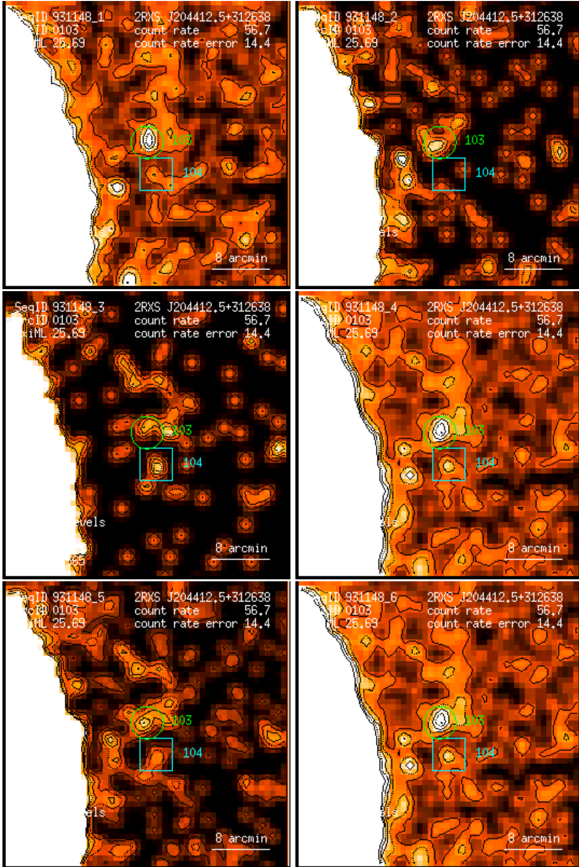
Figure 103: RASS 931148: detection 0103: band rate images, Gaussian filter: (1) PSPC channels 11 – 41, (2) 52 – 90, (3) 91 – 201, (4) 11 – 235, (5) 52 – 201, (6) 11 – 201. Broad band rates in counts/ks. Band rate contour levels in counts/ks/arcmin 2 .
