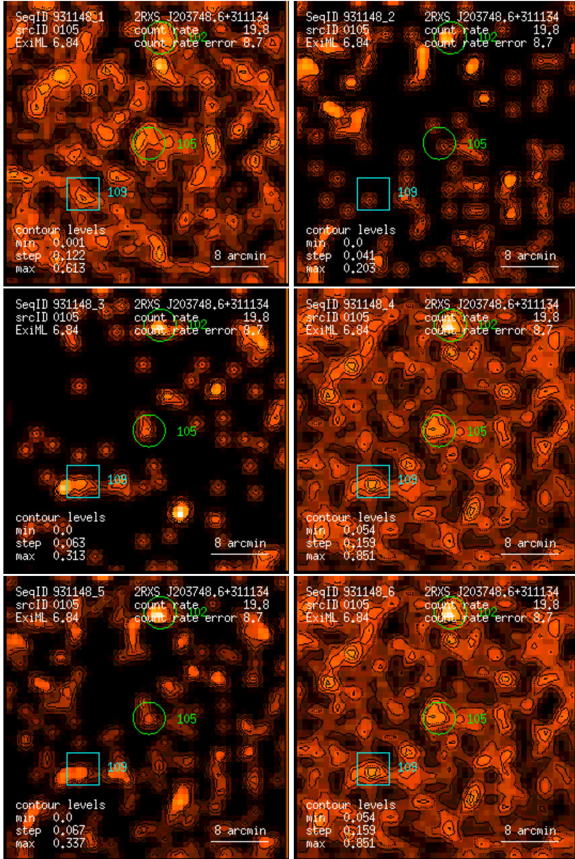
Figure 105: RASS 931148: detection 0105: band rate images, Gaussian filter: (1) PSPC channels 11 – 41, (2) 52 – 90, (3) 91 – 201, (4) 11 – 235, (5) 52 – 201, (6) 11 – 201. Broad band rates in counts/ks. Band rate contour levels in counts/ks/arcmin 2 .
