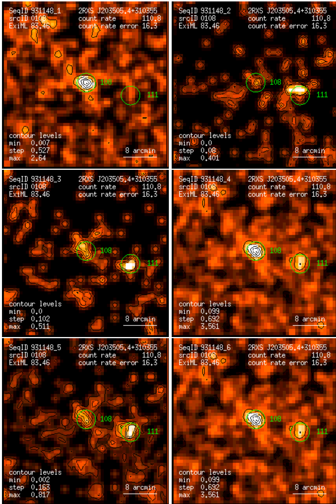
Figure 108: RASS 931148: detection 0108: band rate images, Gaussian filter: (1) PSPC channels 11 – 41, (2) 52 – 90, (3) 91 – 201, (4) 11 – 235, (5) 52 – 201, (6) 11 – 201. Broad band rates in counts/ks. Band rate contour levels in counts/ks/arcmin 2 .
