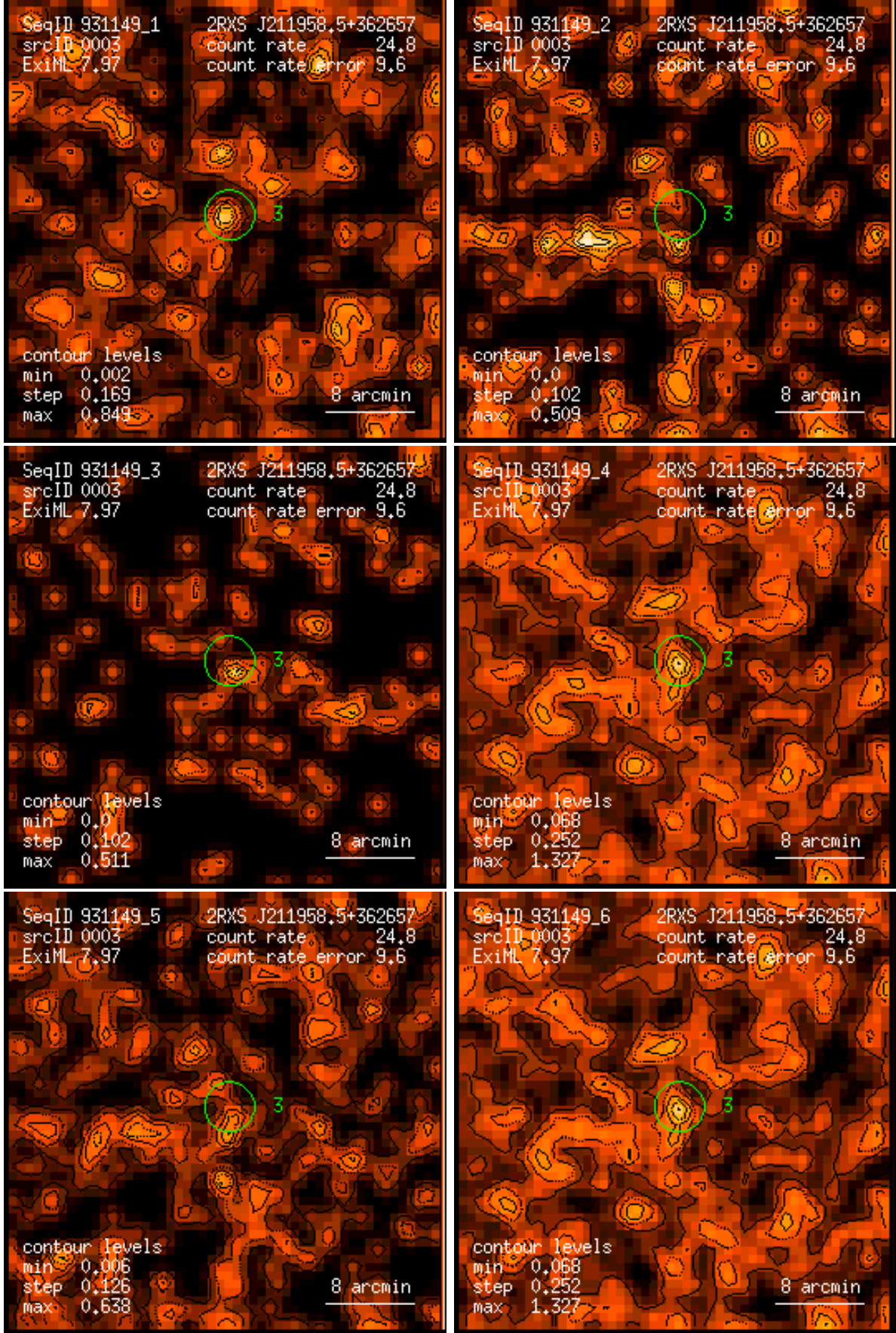
Figure 3: RASS 931149: detection 0003: band rate images, Gaussian filter: (1) PSPC channels 11 – 41, (2) 52 – 90, (3) 91 – 201, (4) 11 – 235, (5) 52 – 201, (6) 11 – 201. Broad band rates in counts/ks. Band rate contour levels in counts/ks/arcmin 2 .
