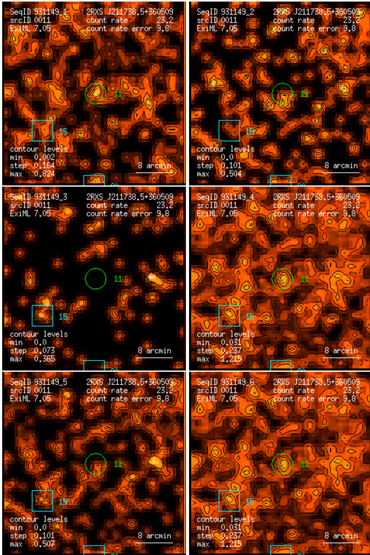
Figure 11: RASS 931149: detection 0011: band rate images, Gaussian filter: (1) PSPC channels 11 – 41, (2) 52 – 90, (3) 91 – 201, (4) 11 – 235, (5) 52 – 201, (6) 11 – 201. Broad band rates in counts/ks. Band rate contour levels in counts/ks/arcmin 2 .
