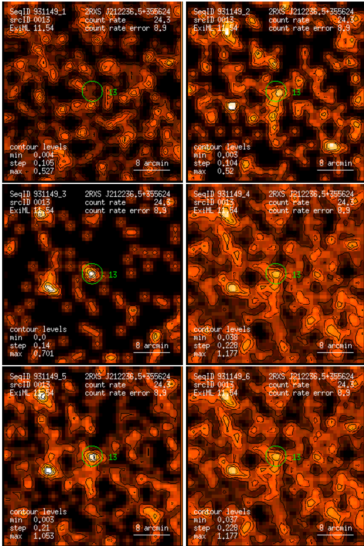
Figure 13: RASS 931149: detection 0013: band rate images, Gaussian filter: (1) PSPC channels 11 – 41, (2) 52 – 90, (3) 91 – 201, (4) 11 – 235, (5) 52 – 201, (6) 11 – 201. Broad band rates in counts/ks. Band rate contour levels in counts/ks/arcmin 2 .
