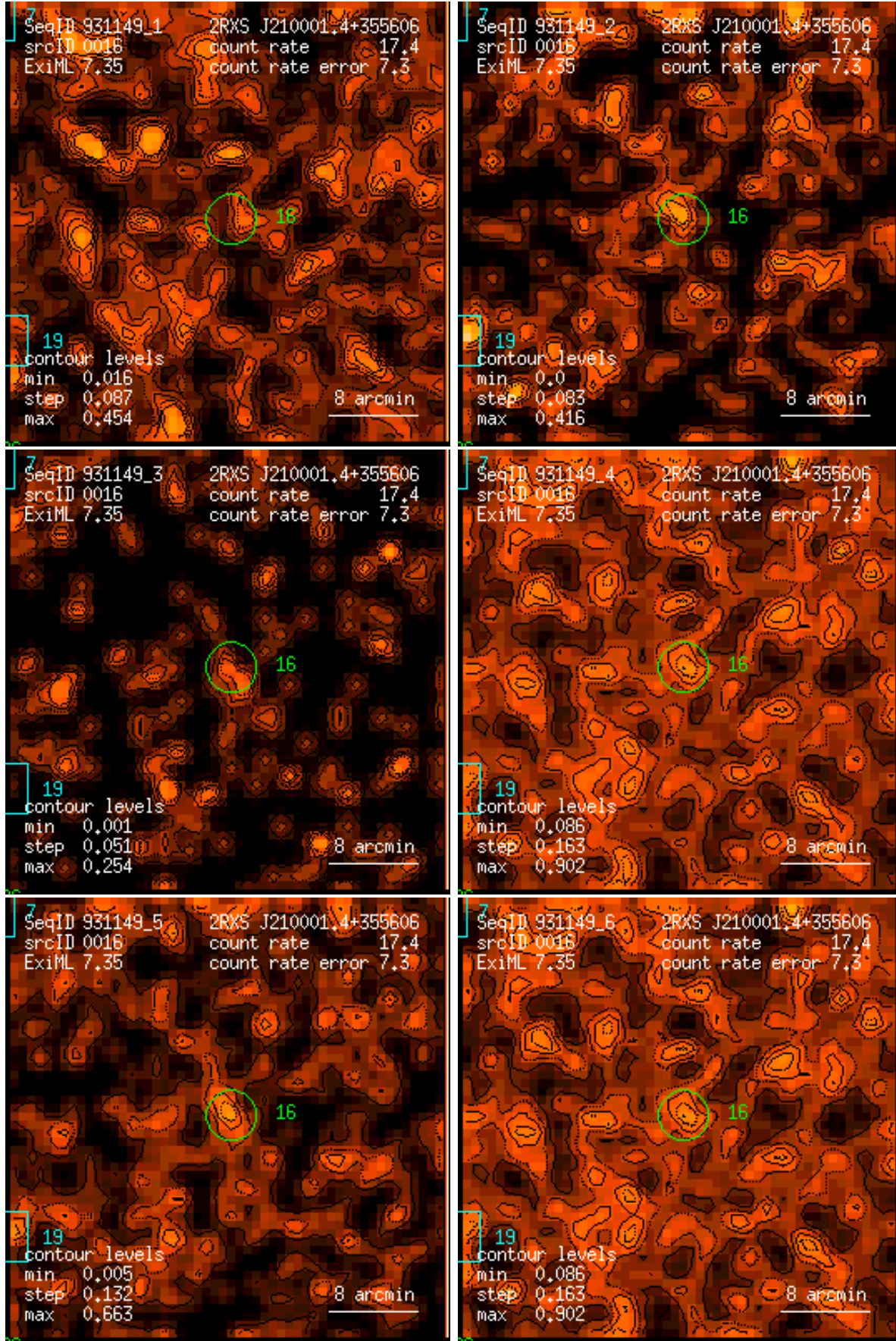
Figure 16: RASS 931149: detection 0016: band rate images, Gaussian filter: (1) PSPC channels 11 – 41, (2) 52 – 90, (3) 91 – 201, (4) 11 – 235, (5) 52 – 201, (6) 11 – 201. Broad band rates in counts/ks. Band rate contour levels in counts/ks/arcmin 2 .
