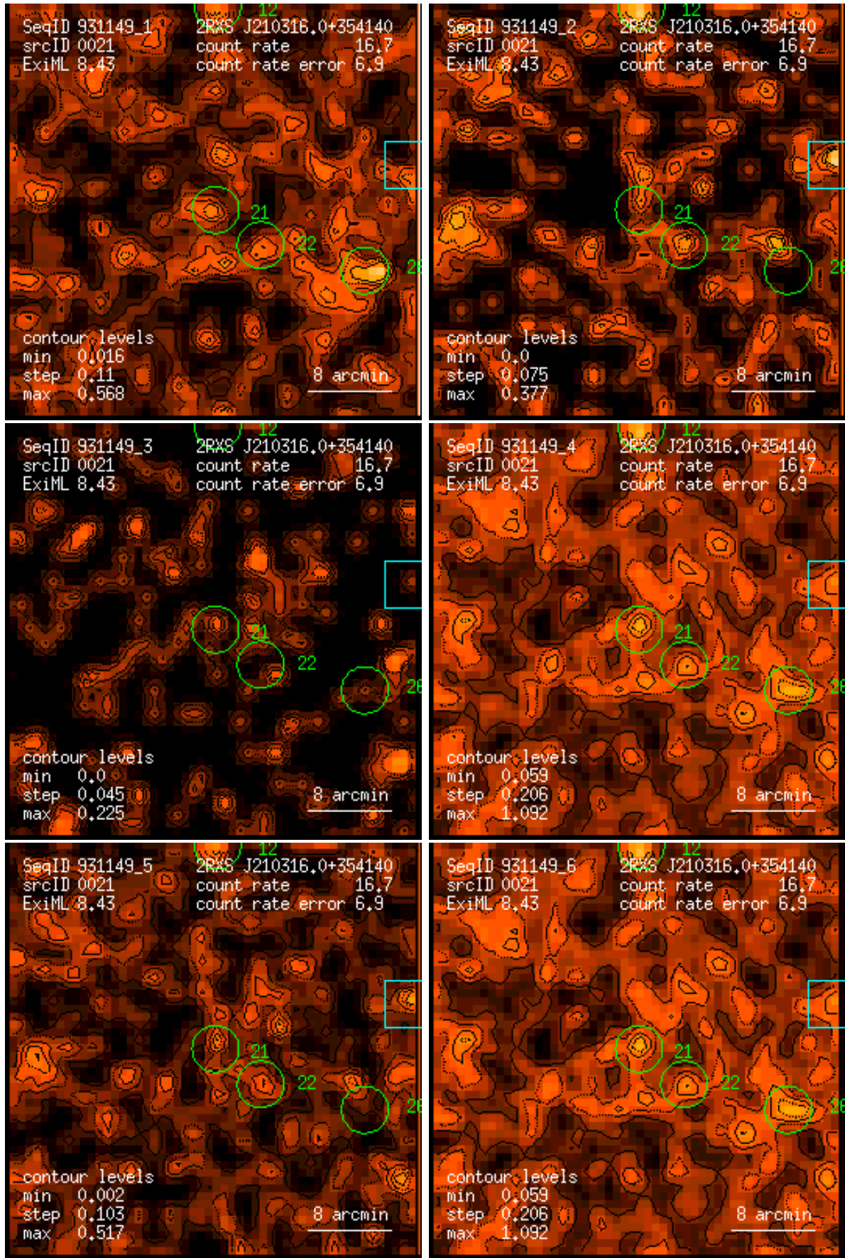
Figure 21: RASS 931149: detection 0021: band rate images, Gaussian filter: (1) PSPC channels 11 – 41, (2) 52 – 90, (3) 91 – 201, (4) 11 – 235, (5) 52 – 201, (6) 11 – 201. Broad band rates in counts/ks. Band rate contour levels in counts/ks/arcmin 2 .
