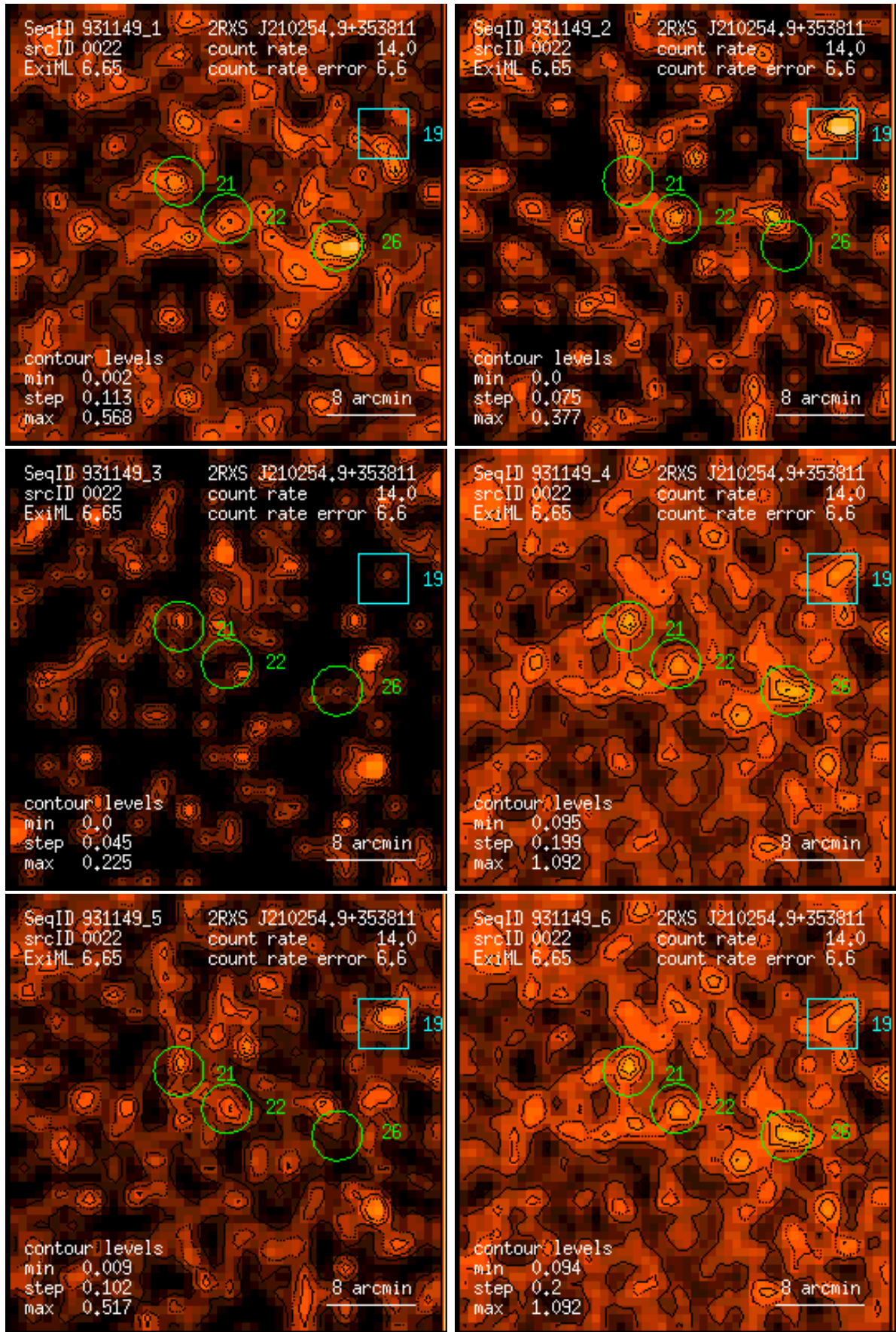
Figure 22: RASS 931149: detection 0022: band rate images, Gaussian filter: (1) PSPC channels 11 – 41, (2) 52 – 90, (3) 91 – 201, (4) 11 – 235, (5) 52 – 201, (6) 11 – 201. Broad band rates in counts/ks. Band rate contour levels in counts/ks/arcmin 2 .
