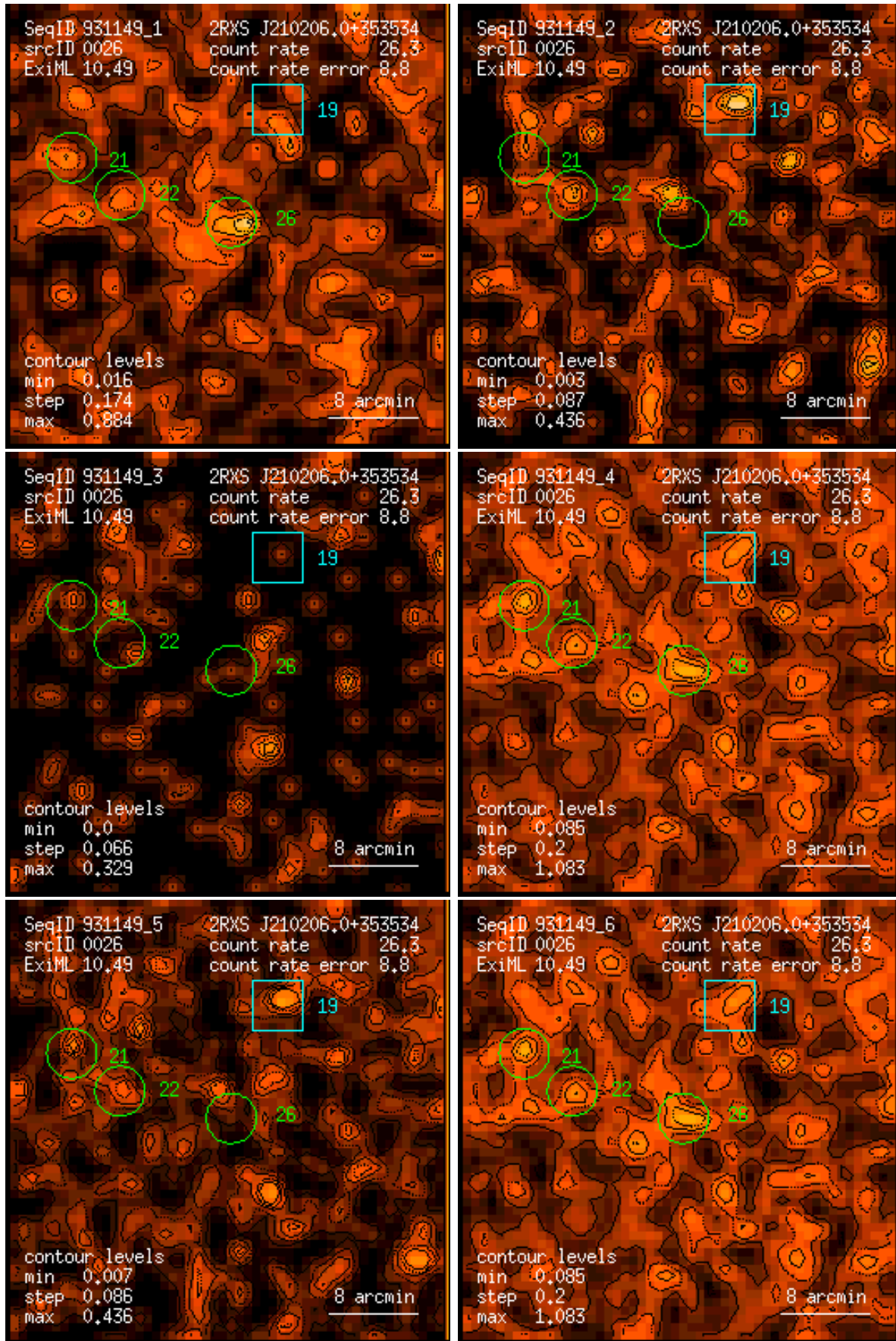
Figure 26: RASS 931149: detection 0026: band rate images, Gaussian filter: (1) PSPC channels 11 – 41, (2) 52 – 90, (3) 91 – 201, (4) 11 – 235, (5) 52 – 201, (6) 11 – 201. Broad band rates in counts/ks. Band rate contour levels in counts/ks/arcmin 2 .
