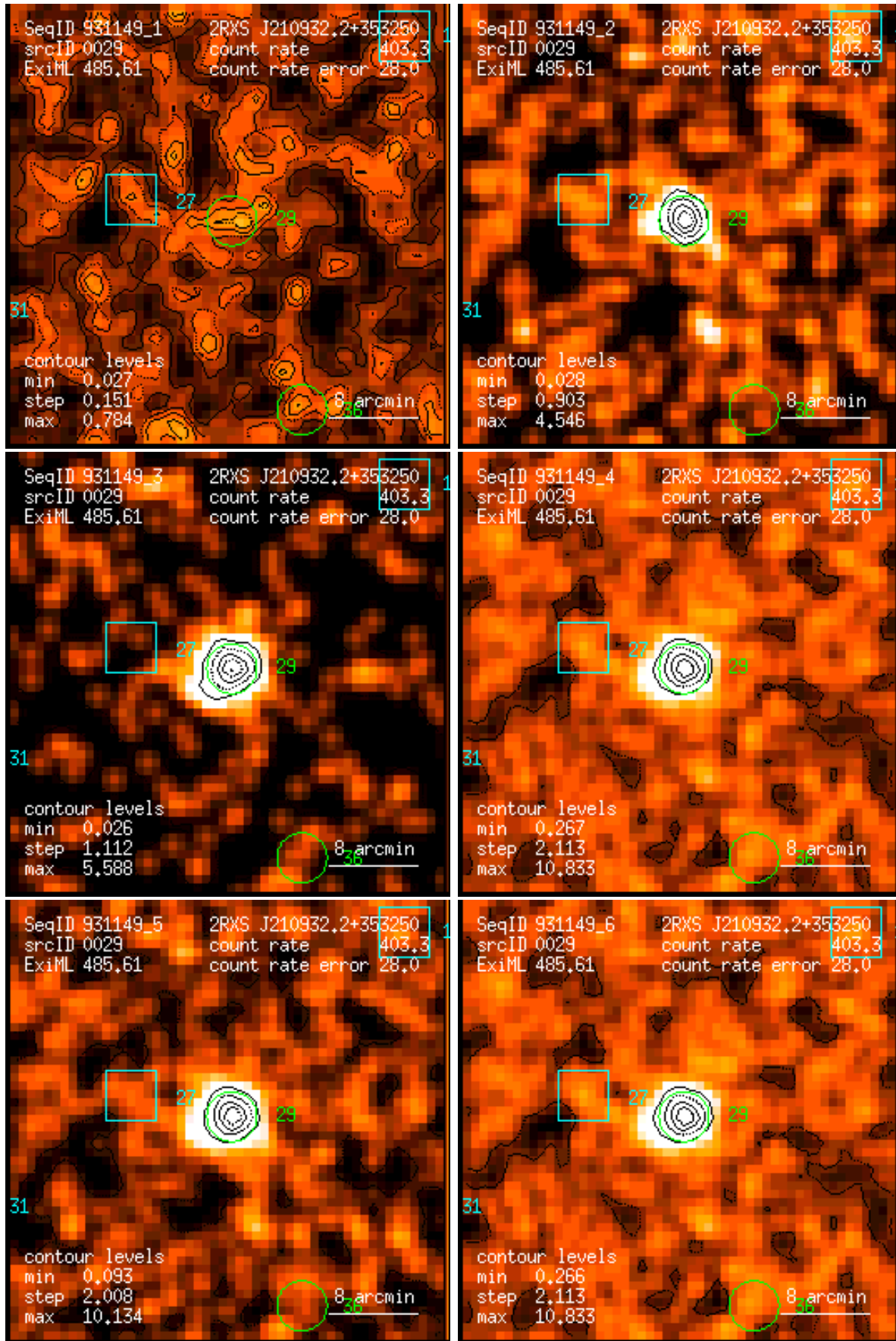
Figure 29: RASS 931149: detection 0029: band rate images, Gaussian filter: (1) PSPC channels 11 – 41, (2) 52 – 90, (3) 91 – 201, (4) 11 – 235, (5) 52 – 201, (6) 11 – 201. Broad band rates in counts/ks. Band rate contour levels in counts/ks/arcmin 2 .
