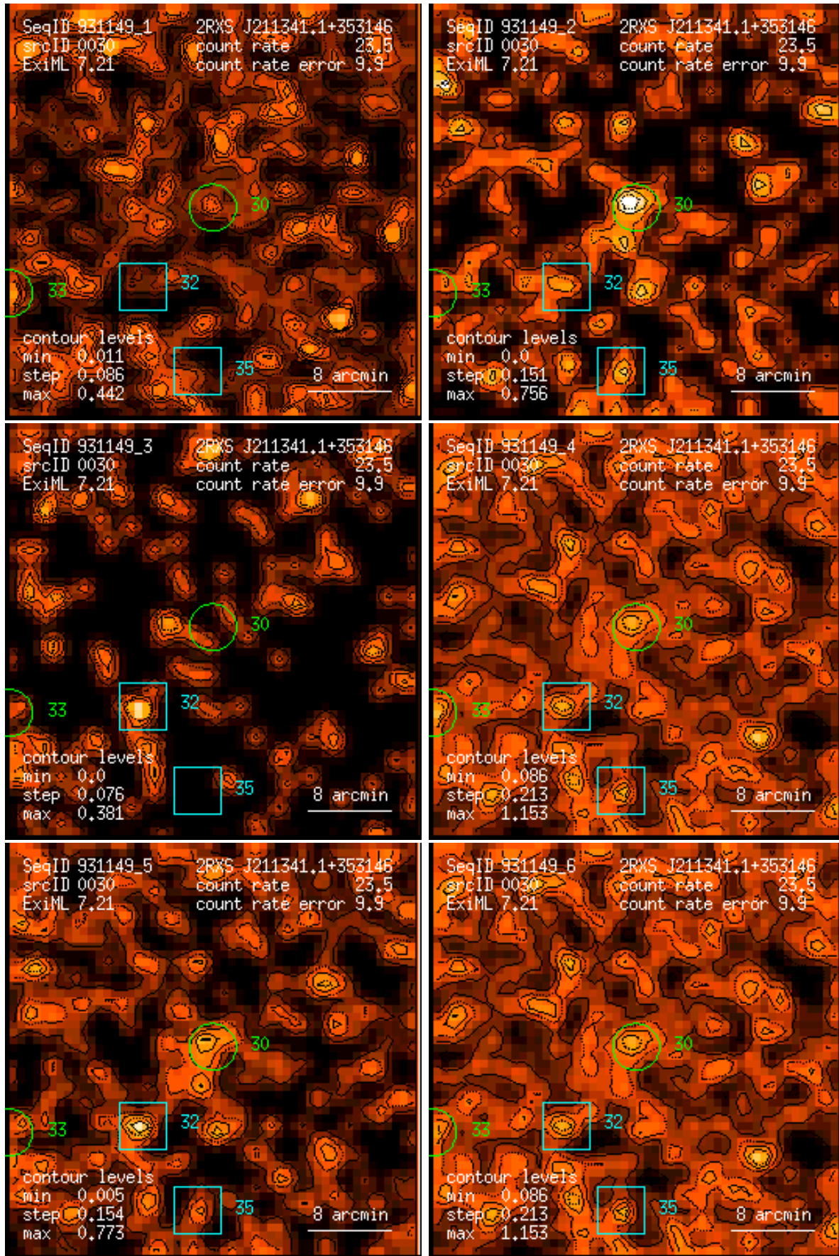
Figure 30: RASS 931149: detection 0030: band rate images, Gaussian filter: (1) PSPC channels 11 – 41, (2) 52 – 90, (3) 91 – 201, (4) 11 – 235, (5) 52 – 201, (6) 11 – 201. Broad band rates in counts/ks. Band rate contour levels in counts/ks/arcmin 2 .
