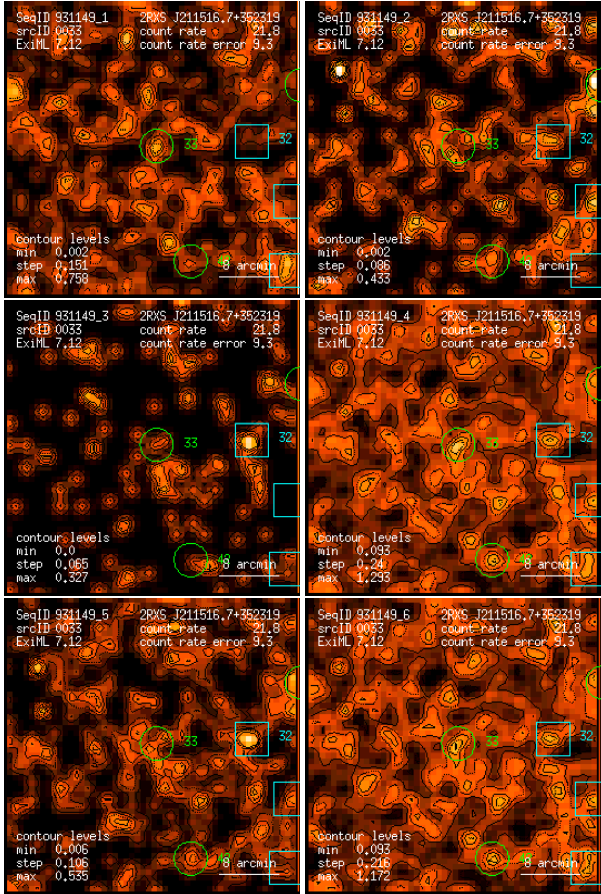
Figure 33: RASS 931149: detection 0033: band rate images, Gaussian filter: (1) PSPC channels 11 – 41, (2) 52 – 90, (3) 91 – 201, (4) 11 – 235, (5) 52 – 201, (6) 11 – 201. Broad band rates in counts/ks. Band rate contour levels in counts/ks/arcmin 2 .
