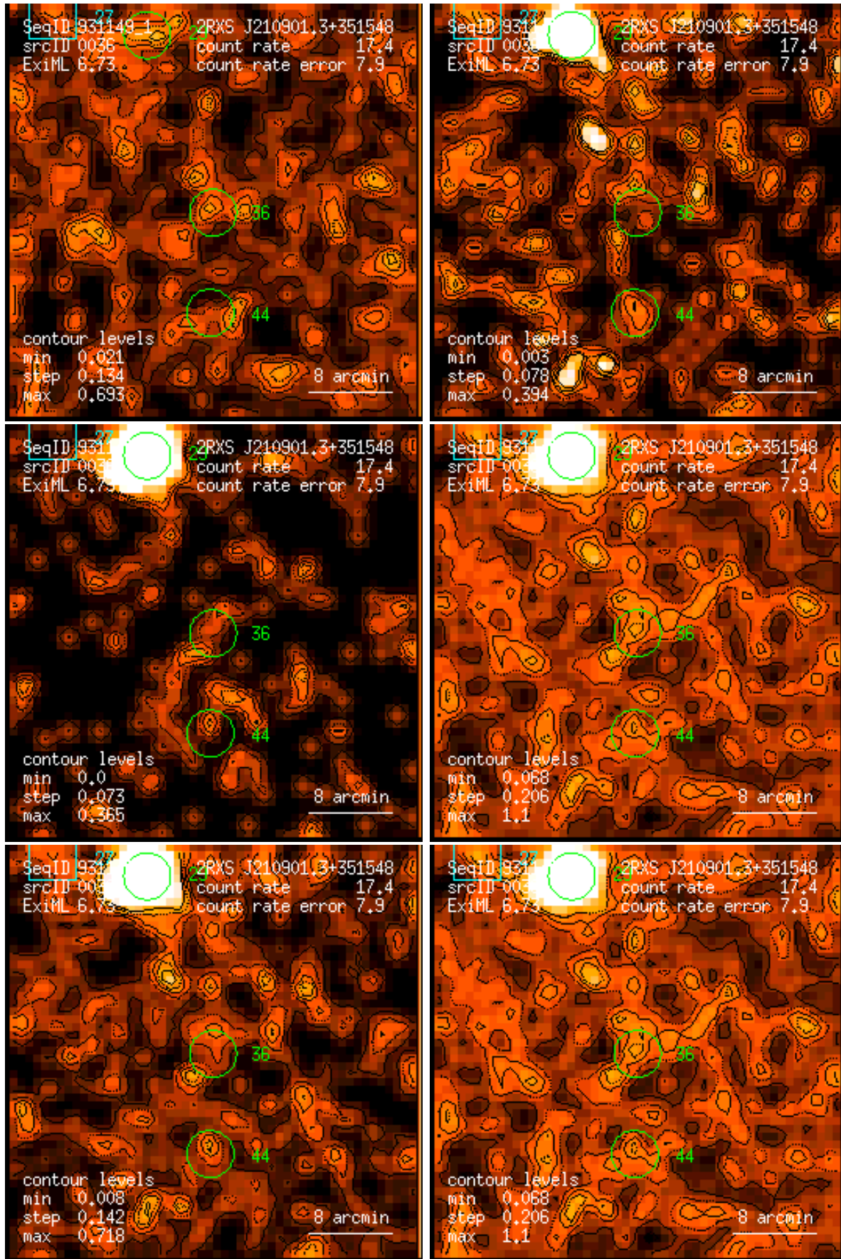
Figure 36: RASS 931149: detection 0036: band rate images, Gaussian filter: (1) PSPC channels 11 – 41, (2) 52 – 90, (3) 91 – 201, (4) 11 – 235, (5) 52 – 201, (6) 11 – 201. Broad band rates in counts/ks. Band rate contour levels in counts/ks/arcmin 2 .
