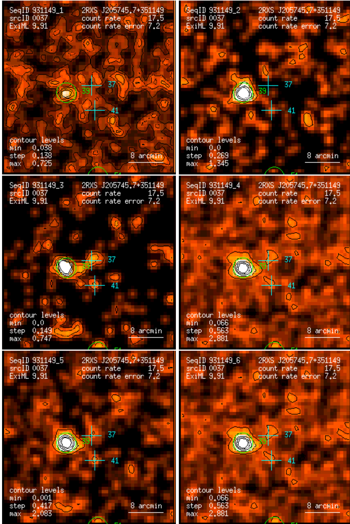
Figure 37: RASS 931149: detection 0037: band rate images, Gaussian filter: (1) PSPC channels 11 – 41, (2) 52 – 90, (3) 91 – 201, (4) 11 – 235, (5) 52 – 201, (6) 11 – 201. Broad band rates in counts/ks. Band rate contour levels in counts/ks/arcmin 2 .
