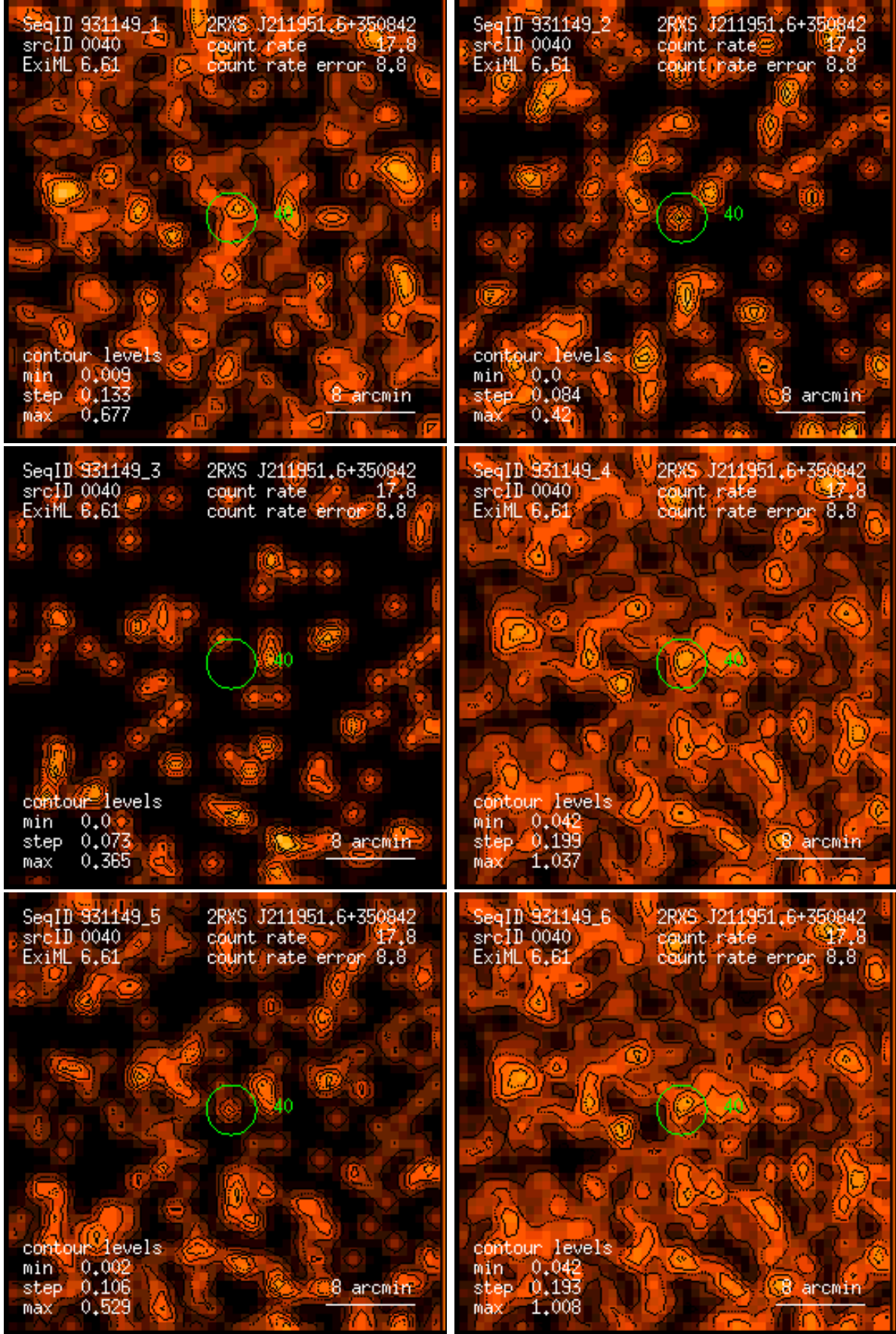
Figure 40: RASS 931149: detection 0040: band rate images, Gaussian filter: (1) PSPC channels 11 – 41, (2) 52 – 90, (3) 91 – 201, (4) 11 – 235, (5) 52 – 201, (6) 11 – 201. Broad band rates in counts/ks. Band rate contour levels in counts/ks/arcmin 2 .
