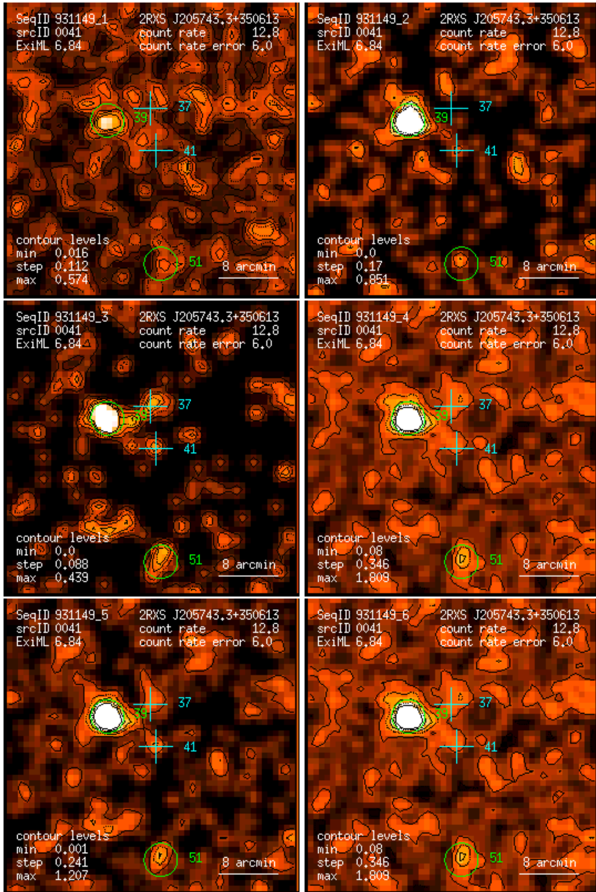
Figure 41: RASS 931149: detection 0041: band rate images, Gaussian filter: (1) PSPC channels 11 – 41, (2) 52 – 90, (3) 91 – 201, (4) 11 – 235, (5) 52 – 201, (6) 11 – 201. Broad band rates in counts/ks. Band rate contour levels in counts/ks/arcmin 2 .
