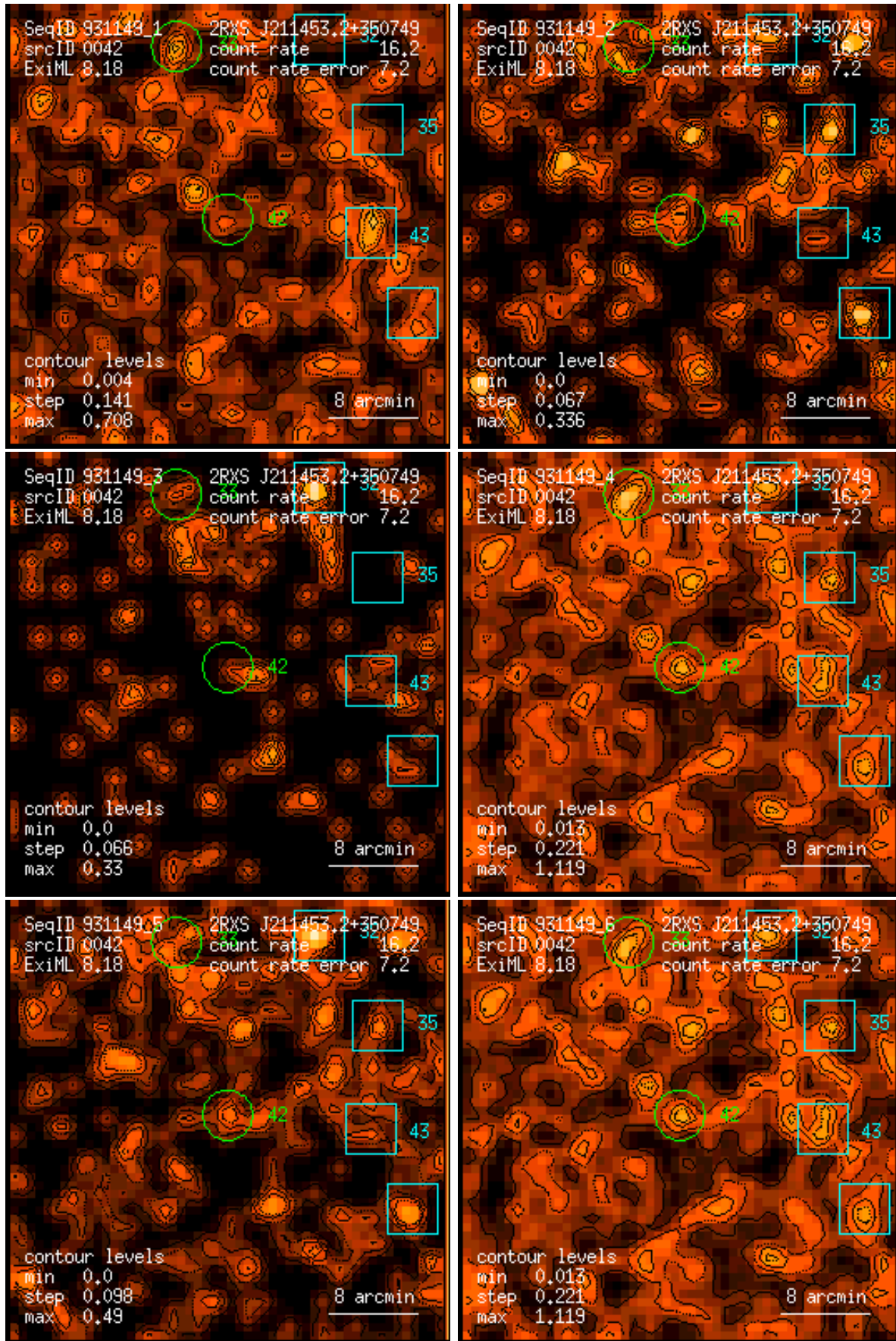
Figure 42: RASS 931149: detection 0042: band rate images, Gaussian filter: (1) PSPC channels 11 – 41, (2) 52 – 90, (3) 91 – 201, (4) 11 – 235, (5) 52 – 201, (6) 11 – 201. Broad band rates in counts/ks. Band rate contour levels in counts/ks/arcmin 2 .
