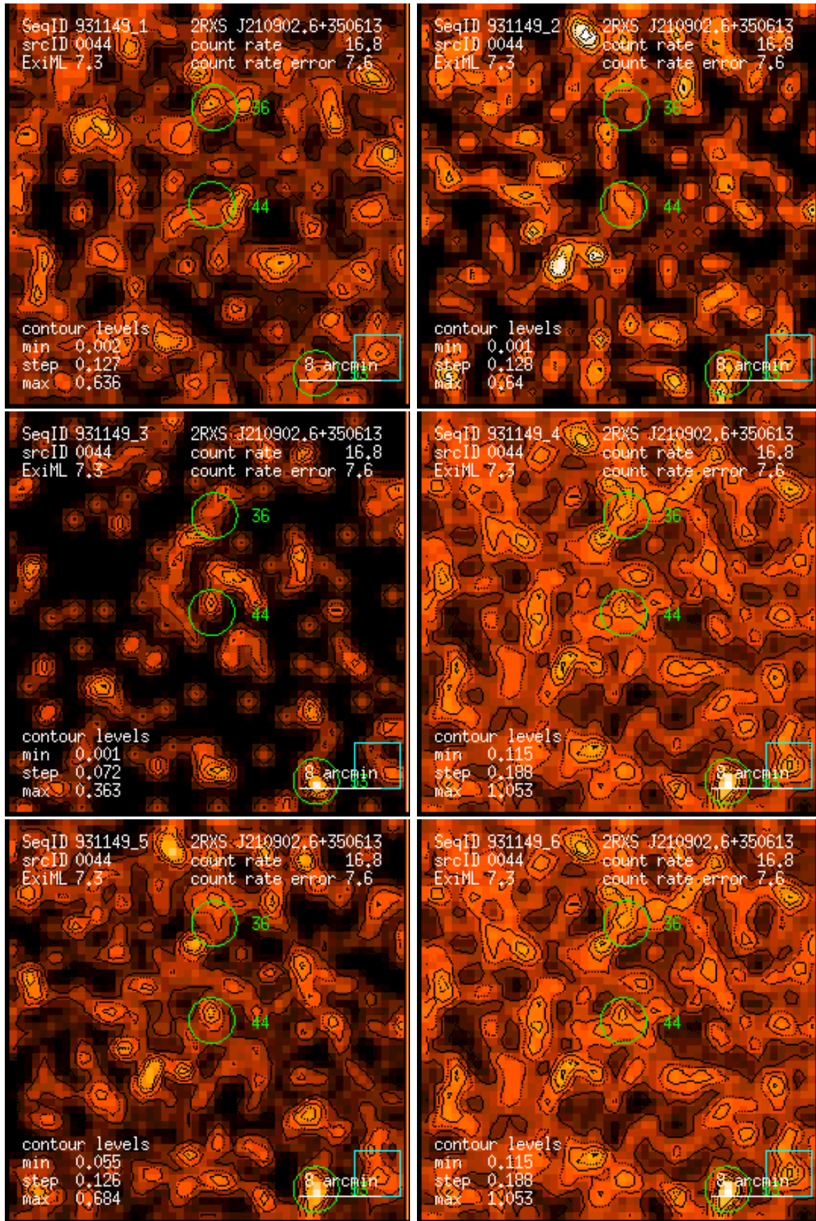
Figure 44: RASS 931149: detection 0044: band rate images, Gaussian filter: (1) PSPC channels 11 – 41, (2) 52 – 90, (3) 91 – 201, (4) 11 – 235, (5) 52 – 201, (6) 11 – 201. Broad band rates in counts/ks. Band rate contour levels in counts/ks/arcmin 2 .
