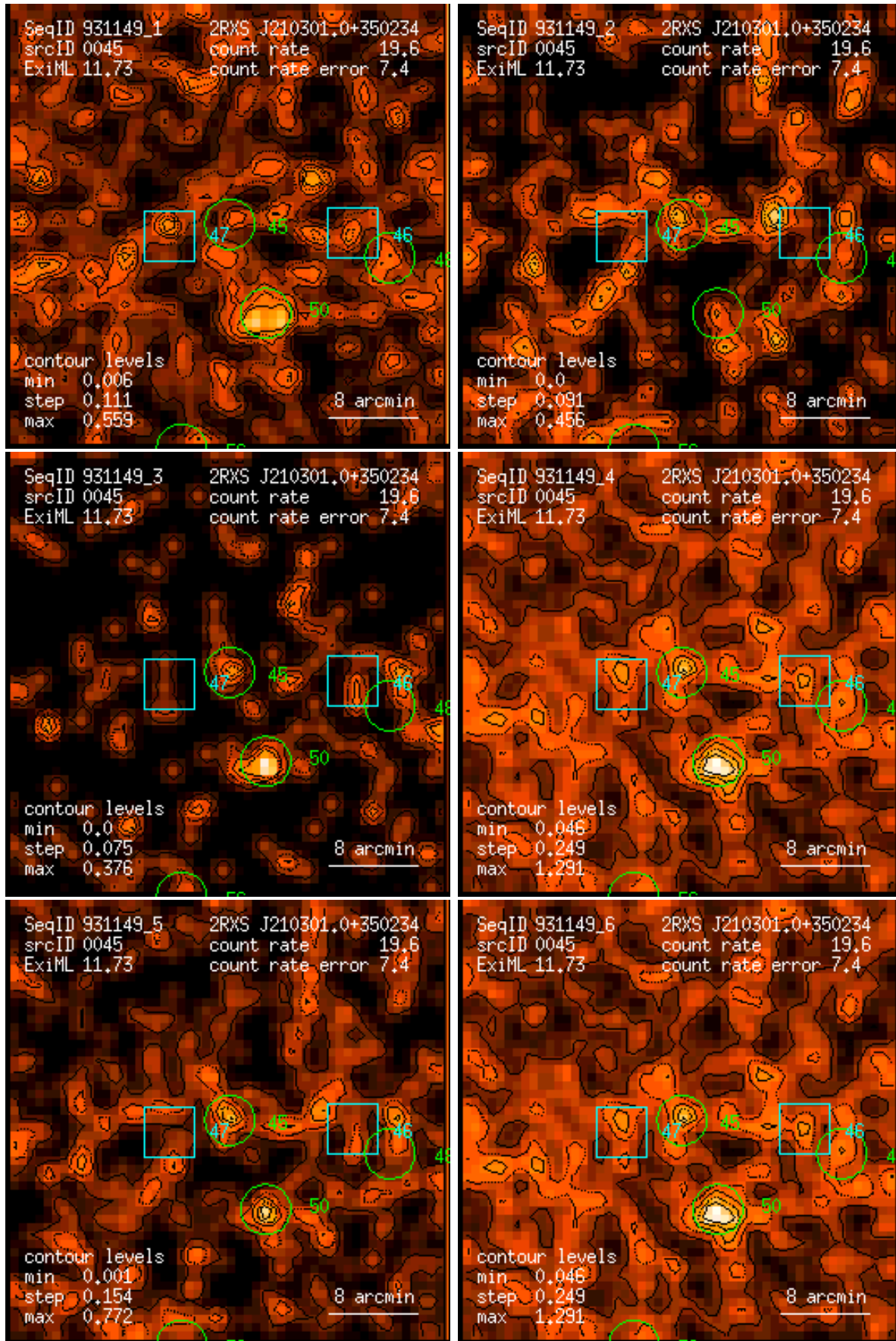
Figure 45: RASS 931149: detection 0045: band rate images, Gaussian filter: (1) PSPC channels 11 – 41, (2) 52 – 90, (3) 91 – 201, (4) 11 – 235, (5) 52 – 201, (6) 11 – 201. Broad band rates in counts/ks. Band rate contour levels in counts/ks/arcmin 2 .
