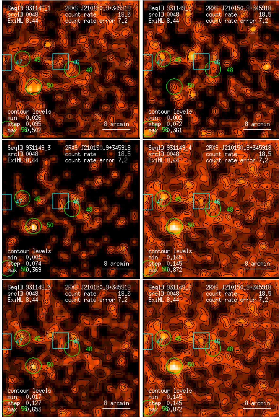
Figure 48: RASS 931149: detection 0048: band rate images, Gaussian filter: (1) PSPC channels 11 – 41, (2) 52 – 90, (3) 91 – 201, (4) 11 – 235, (5) 52 – 201, (6) 11 – 201. Broad band rates in counts/ks. Band rate contour levels in counts/ks/arcmin 2 .
