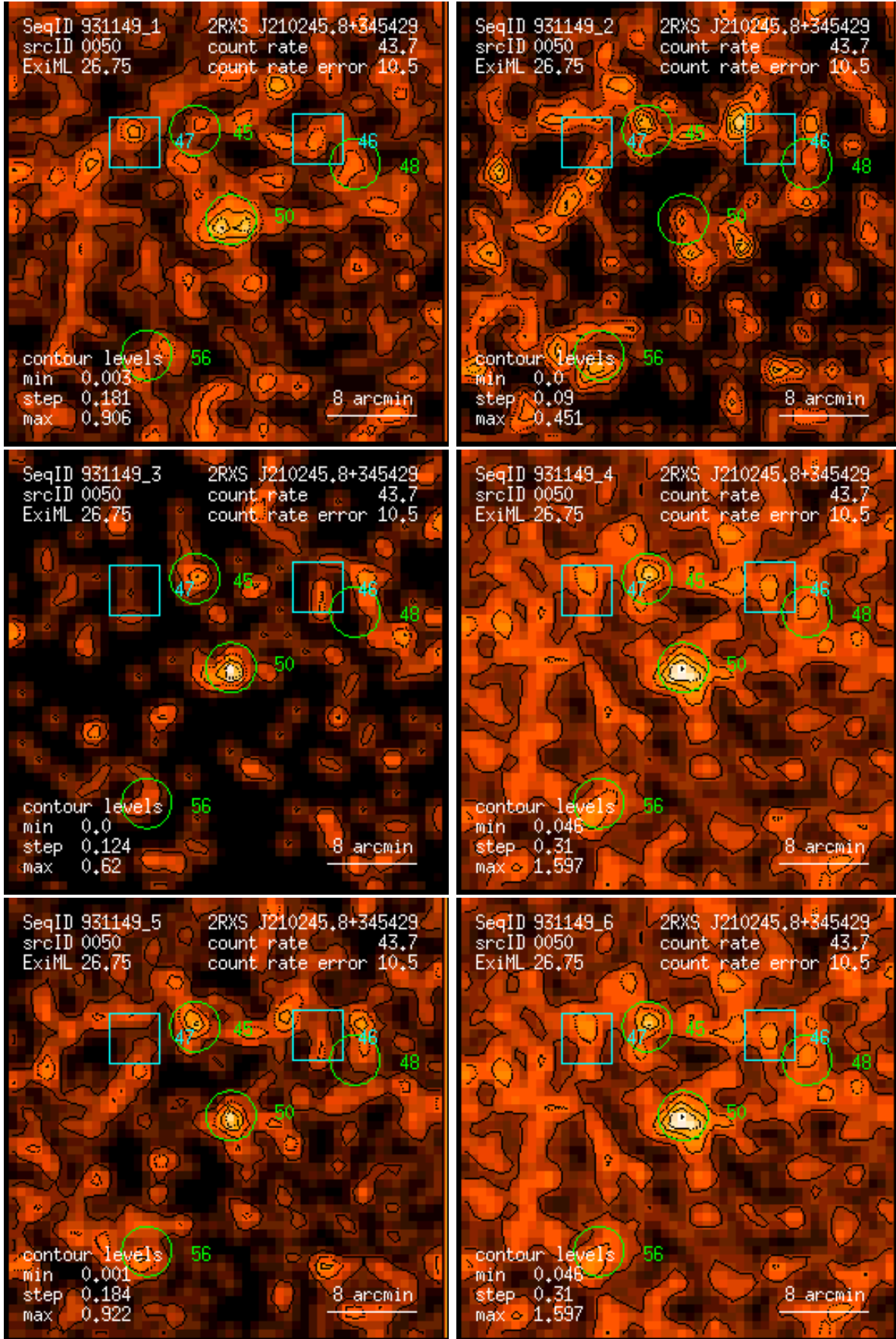
Figure 50: RASS 931149: detection 0050: band rate images, Gaussian filter: (1) PSPC channels 11 – 41, (2) 52 – 90, (3) 91 – 201, (4) 11 – 235, (5) 52 – 201, (6) 11 – 201. Broad band rates in counts/ks. Band rate contour levels in counts/ks/arcmin 2 .
