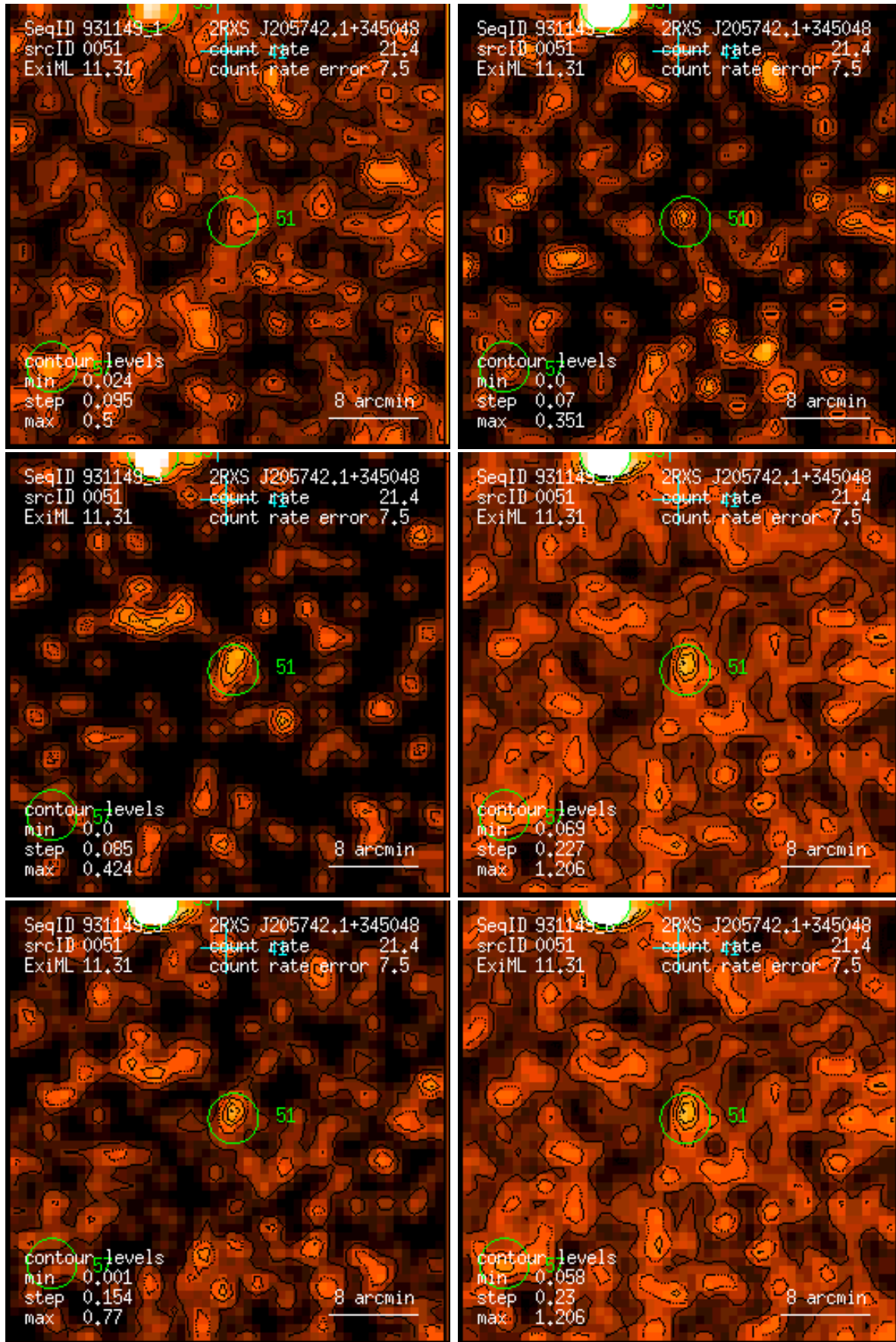
Figure 51: RASS 931149: detection 0051: band rate images, Gaussian filter: (1) PSPC channels 11 – 41, (2) 52 – 90, (3) 91 – 201, (4) 11 – 235, (5) 52 – 201, (6) 11 – 201. Broad band rates in counts/ks. Band rate contour levels in counts/ks/arcmin 2 .
