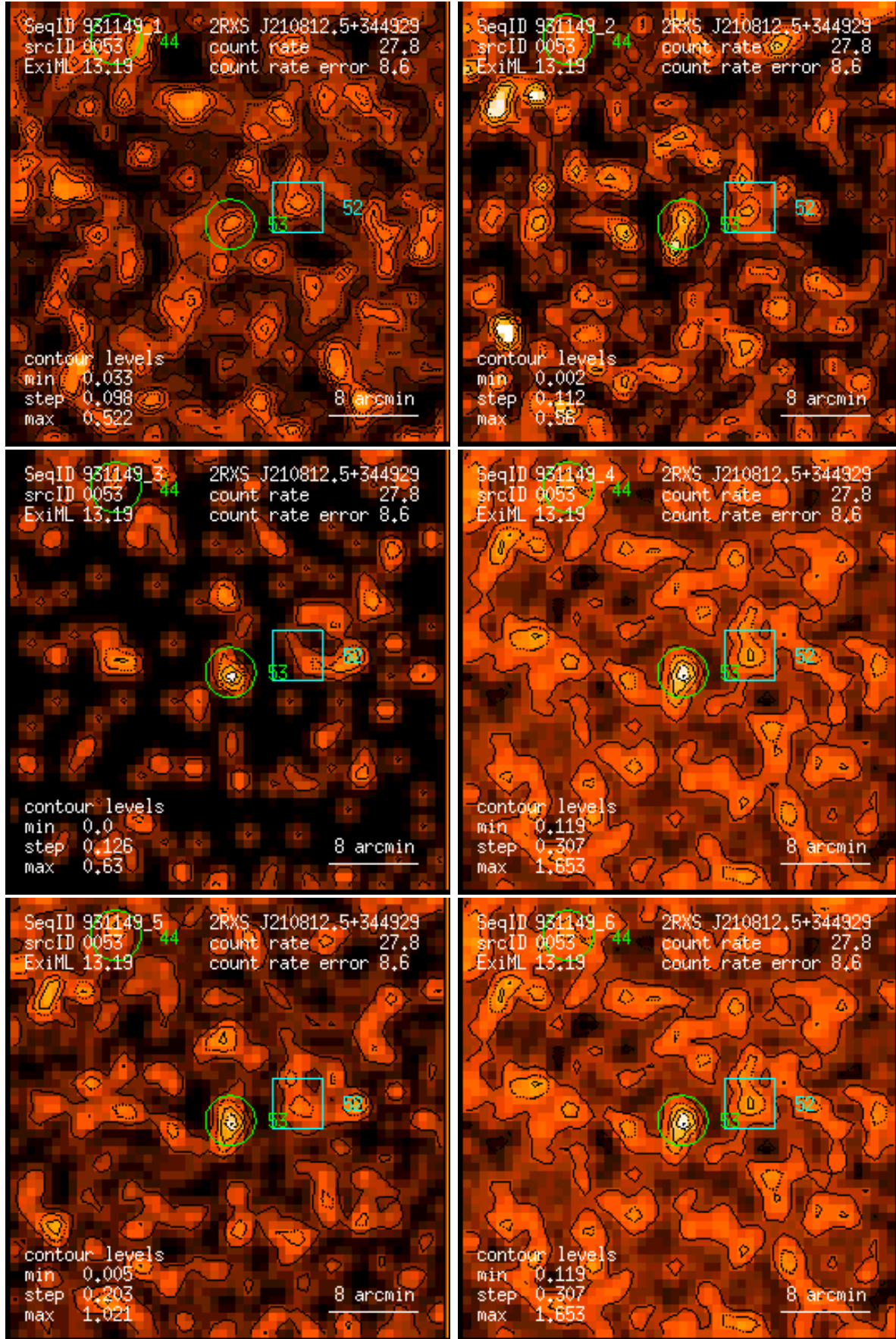
Figure 53: RASS 931149: detection 0053: band rate images, Gaussian filter: (1) PSPC channels 11 – 41, (2) 52 – 90, (3) 91 – 201, (4) 11 – 235, (5) 52 – 201, (6) 11 – 201. Broad band rates in counts/ks. Band rate contour levels in counts/ks/arcmin 2 .
