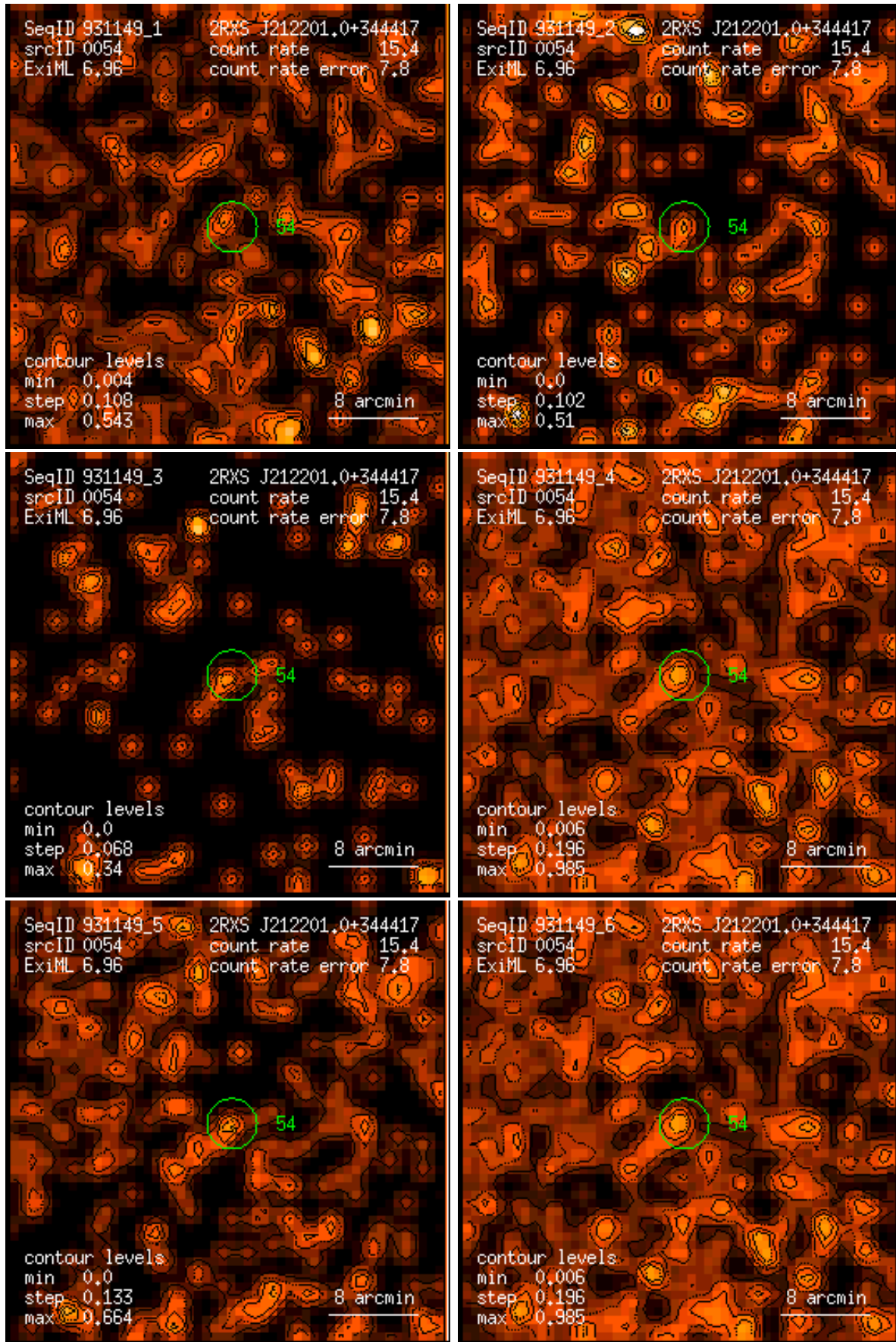
Figure 54: RASS 931149: detection 0054: band rate images, Gaussian filter: (1) PSPC channels 11 – 41, (2) 52 – 90, (3) 91 – 201, (4) 11 – 235, (5) 52 – 201, (6) 11 – 201. Broad band rates in counts/ks. Band rate contour levels in counts/ks/arcmin 2 .
