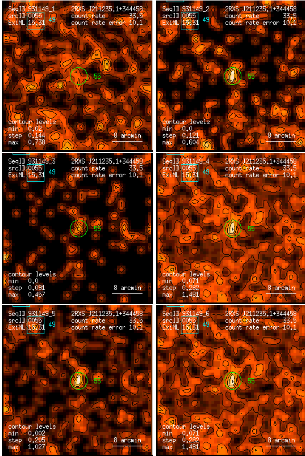
Figure 55: RASS 931149: detection 0055: band rate images, Gaussian filter: (1) PSPC channels 11 – 41, (2) 52 – 90, (3) 91 – 201, (4) 11 – 235, (5) 52 – 201, (6) 11 – 201. Broad band rates in counts/ks. Band rate contour levels in counts/ks/arcmin 2 .
