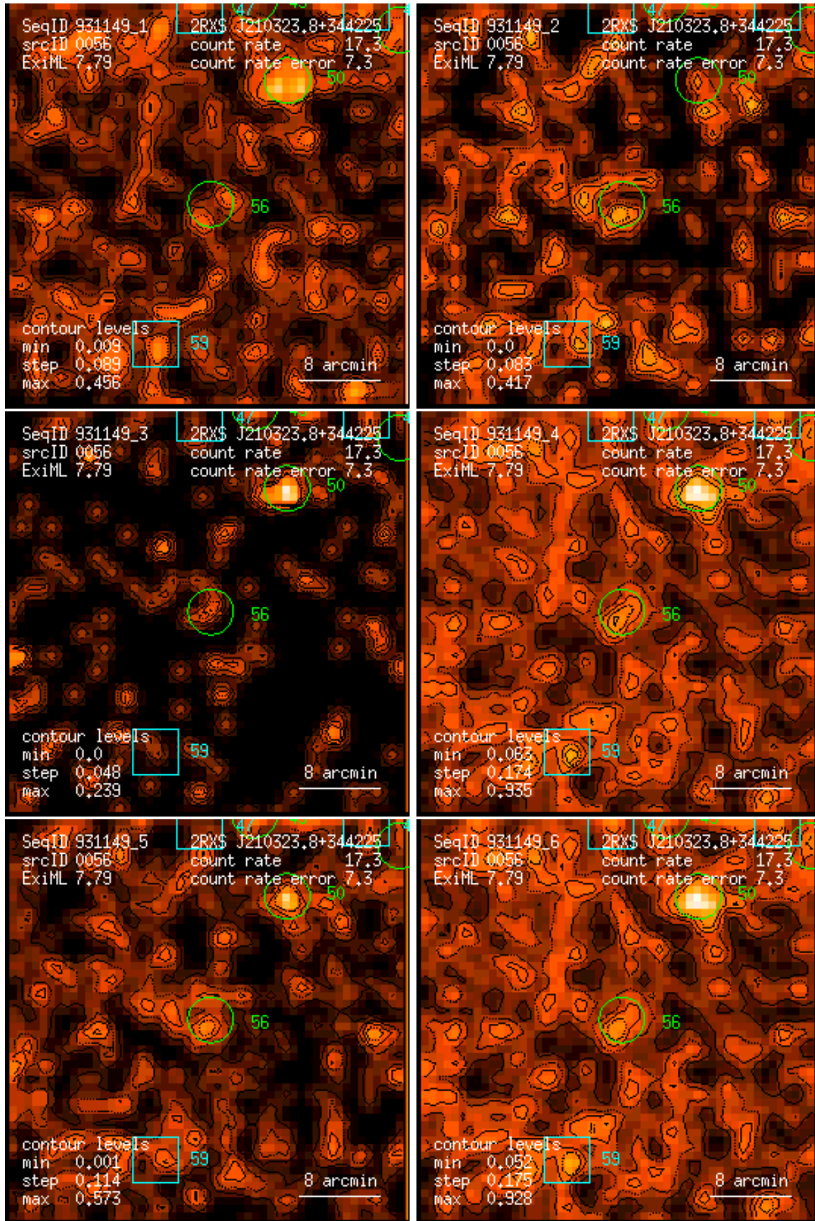
Figure 56: RASS 931149: detection 0056: band rate images, Gaussian filter: (1) PSPC channels 11 – 41, (2) 52 – 90, (3) 91 – 201, (4) 11 – 235, (5) 52 – 201, (6) 11 – 201. Broad band rates in counts/ks. Band rate contour levels in counts/ks/arcmin 2 .
