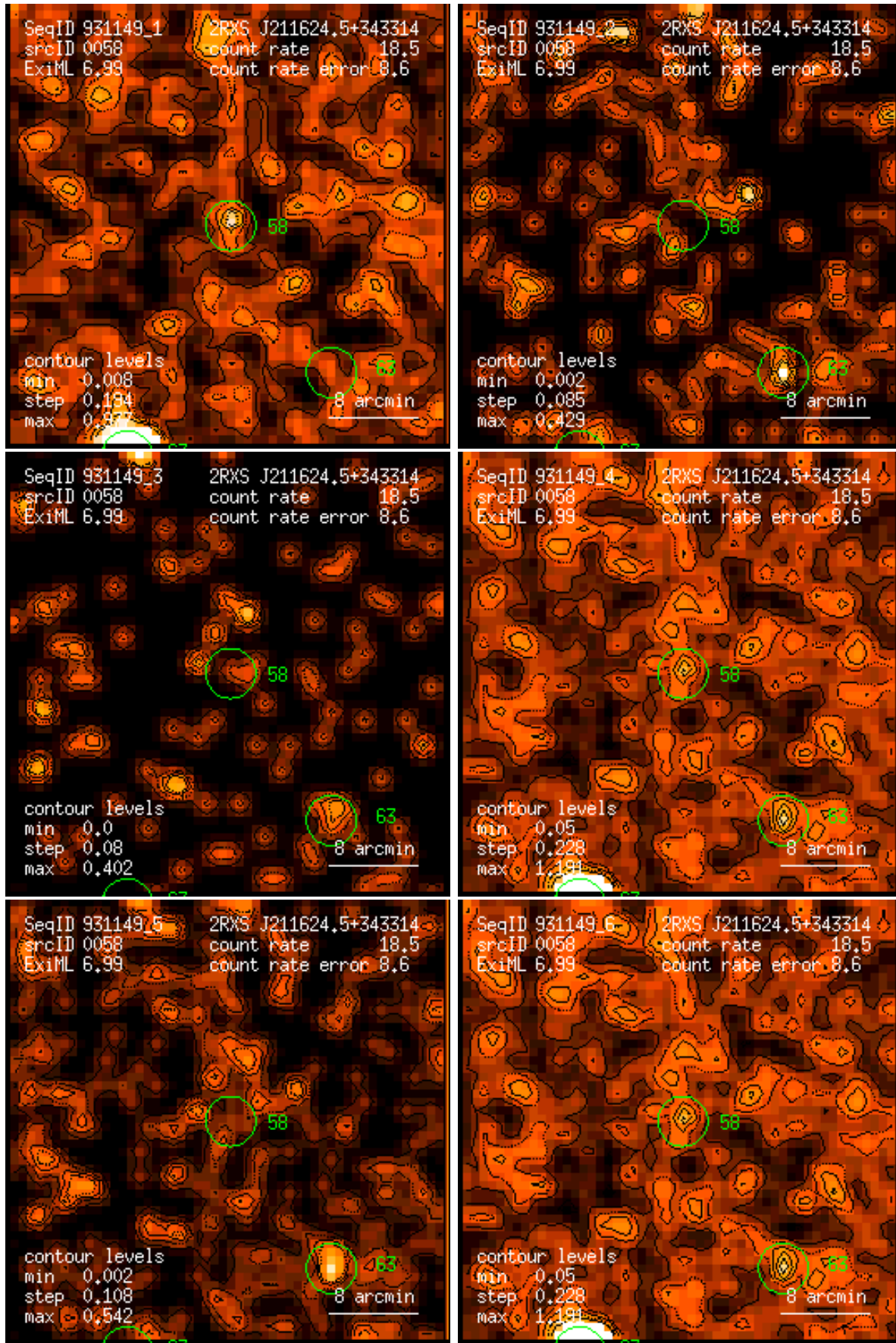
Figure 58: RASS 931149: detection 0058: band rate images, Gaussian filter: (1) PSPC channels 11 – 41, (2) 52 – 90, (3) 91 – 201, (4) 11 – 235, (5) 52 – 201, (6) 11 – 201. Broad band rates in counts/ks. Band rate contour levels in counts/ks/arcmin 2 .
