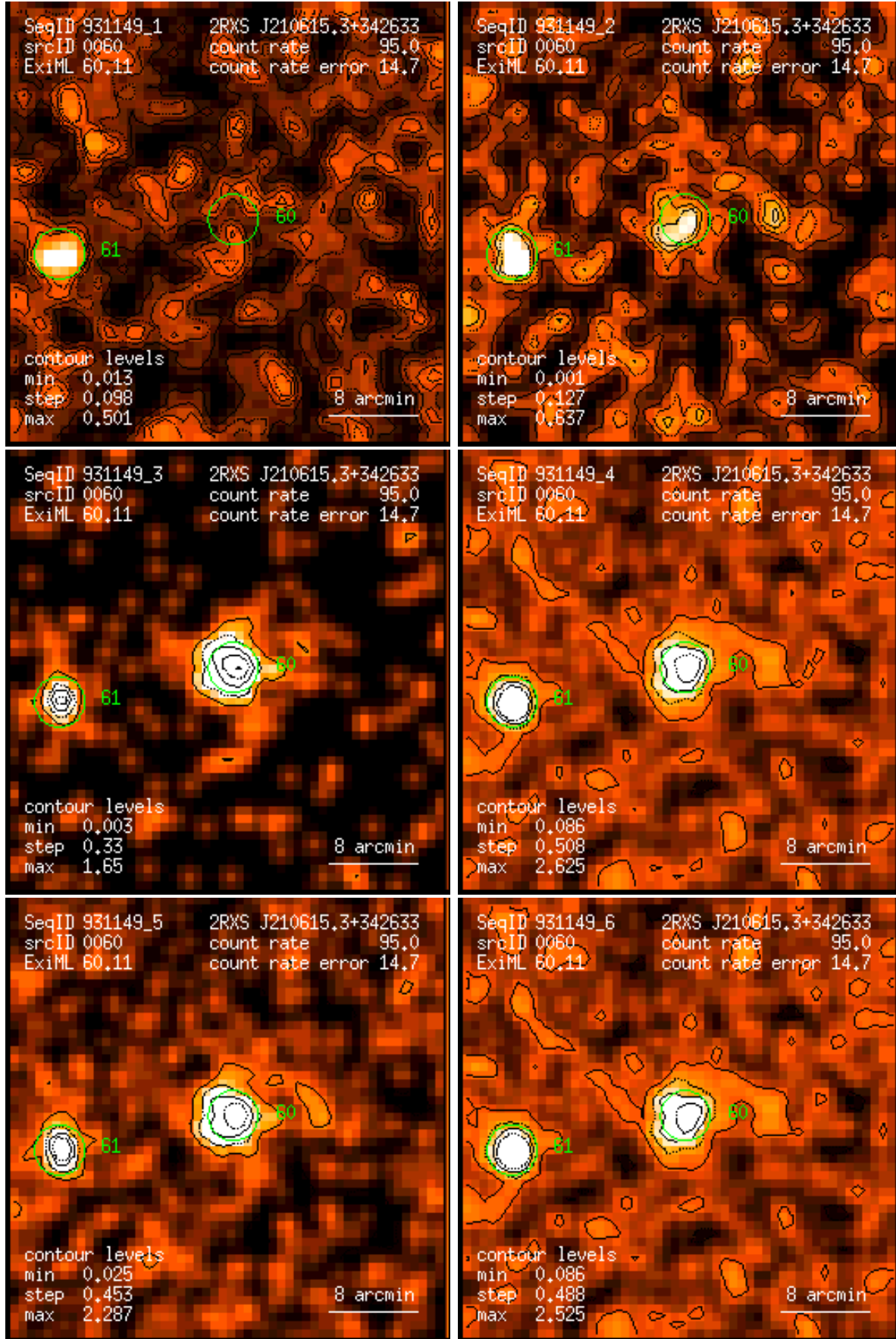
Figure 60: RASS 931149: detection 0060: band rate images, Gaussian filter: (1) PSPC channels 11 – 41, (2) 52 – 90, (3) 91 – 201, (4) 11 – 235, (5) 52 – 201, (6) 11 – 201. Broad band rates in counts/ks. Band rate contour levels in counts/ks/arcmin 2 .
