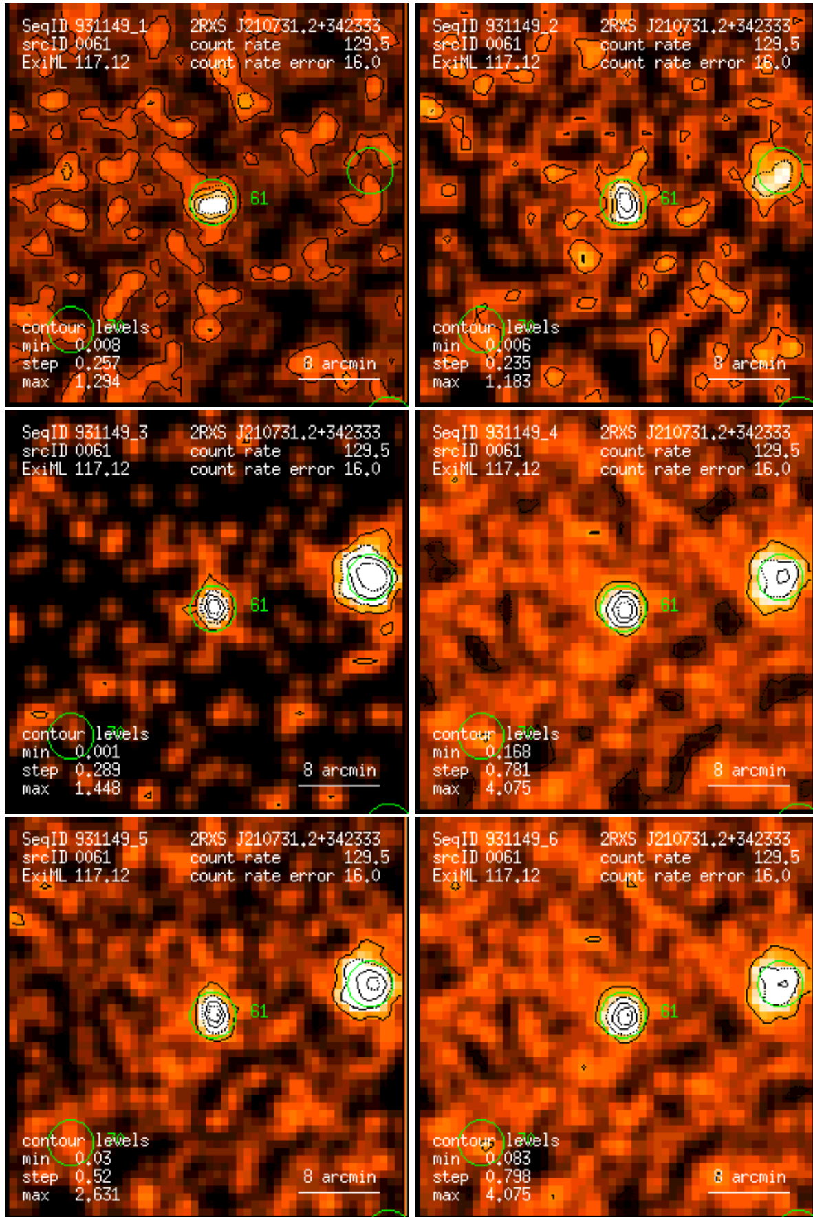
Figure 61: RASS 931149: detection 0061: band rate images, Gaussian filter: (1) PSPC channels 11 – 41, (2) 52 – 90, (3) 91 – 201, (4) 11 – 235, (5) 52 – 201, (6) 11 – 201. Broad band rates in counts/ks. Band rate contour levels in counts/ks/arcmin 2 .
