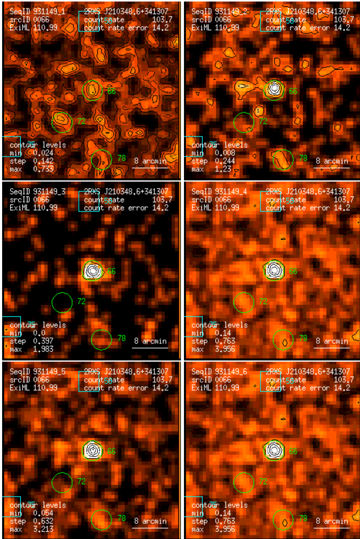
Figure 66: RASS 931149: detection 0066: band rate images, Gaussian filter: (1) PSPC channels 11 – 41, (2) 52 – 90, (3) 91 – 201, (4) 11 – 235, (5) 52 – 201, (6) 11 – 201. Broad band rates in counts/ks. Band rate contour levels in counts/ks/arcmin 2 .
