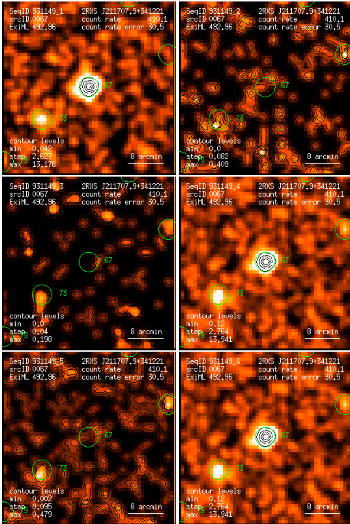
Figure 67: RASS 931149: detection 0067: band rate images, Gaussian filter: (1) PSPC channels 11 – 41, (2) 52 – 90, (3) 91 – 201, (4) 11 – 235, (5) 52 – 201, (6) 11 – 201. Broad band rates in counts/ks. Band rate contour levels in counts/ks/arcmin 2 .
