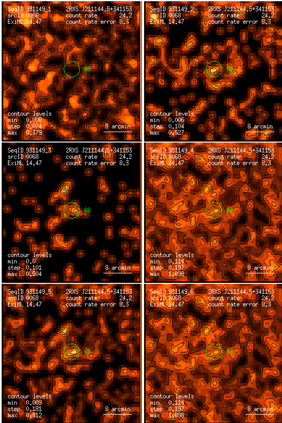
Figure 68: RASS 931149: detection 0068: band rate images, Gaussian filter: (1) PSPC channels 11 – 41, (2) 52 – 90, (3) 91 – 201, (4) 11 – 235, (5) 52 – 201, (6) 11 – 201. Broad band rates in counts/ks. Band rate contour levels in counts/ks/arcmin 2 .
