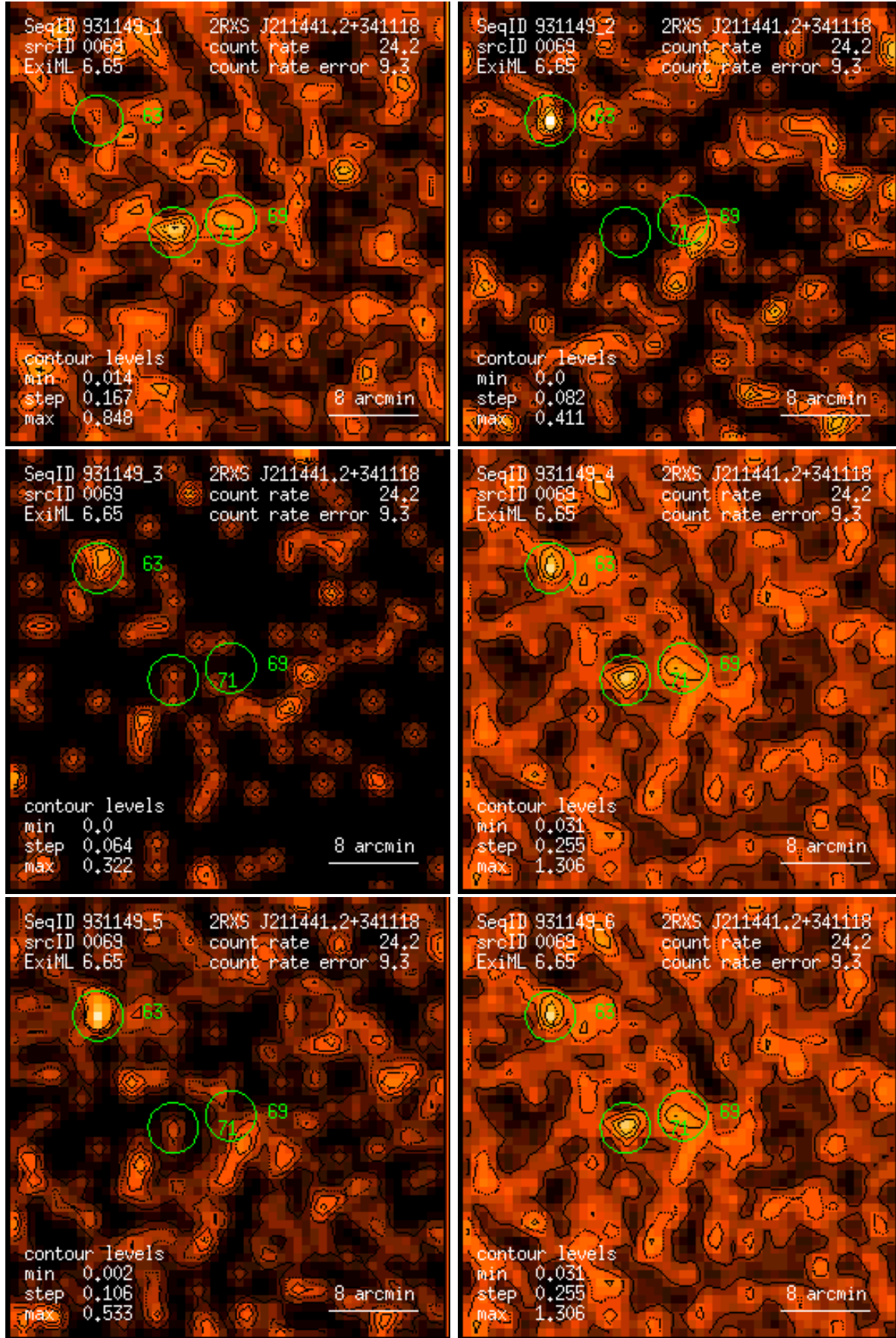
Figure 69: RASS 931149: detection 0069: band rate images, Gaussian filter: (1) PSPC channels 11 – 41, (2) 52 – 90, (3) 91 – 201, (4) 11 – 235, (5) 52 – 201, (6) 11 – 201. Broad band rates in counts/ks. Band rate contour levels in counts/ks/arcmin 2 .
