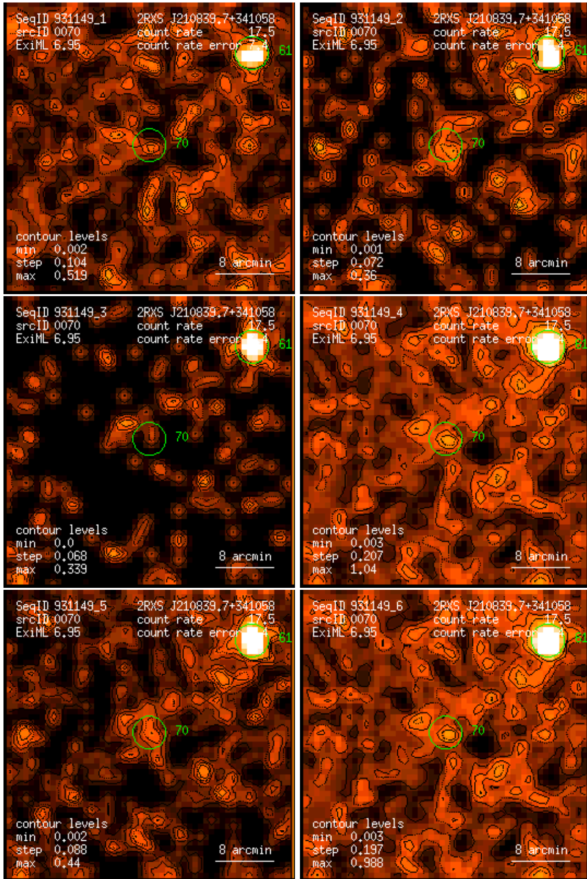
Figure 70: RASS 931149: detection 0070: band rate images, Gaussian filter: (1) PSPC channels 11 – 41, (2) 52 – 90, (3) 91 – 201, (4) 11 – 235, (5) 52 – 201, (6) 11 – 201. Broad band rates in counts/ks. Band rate contour levels in counts/ks/arcmin 2 .
