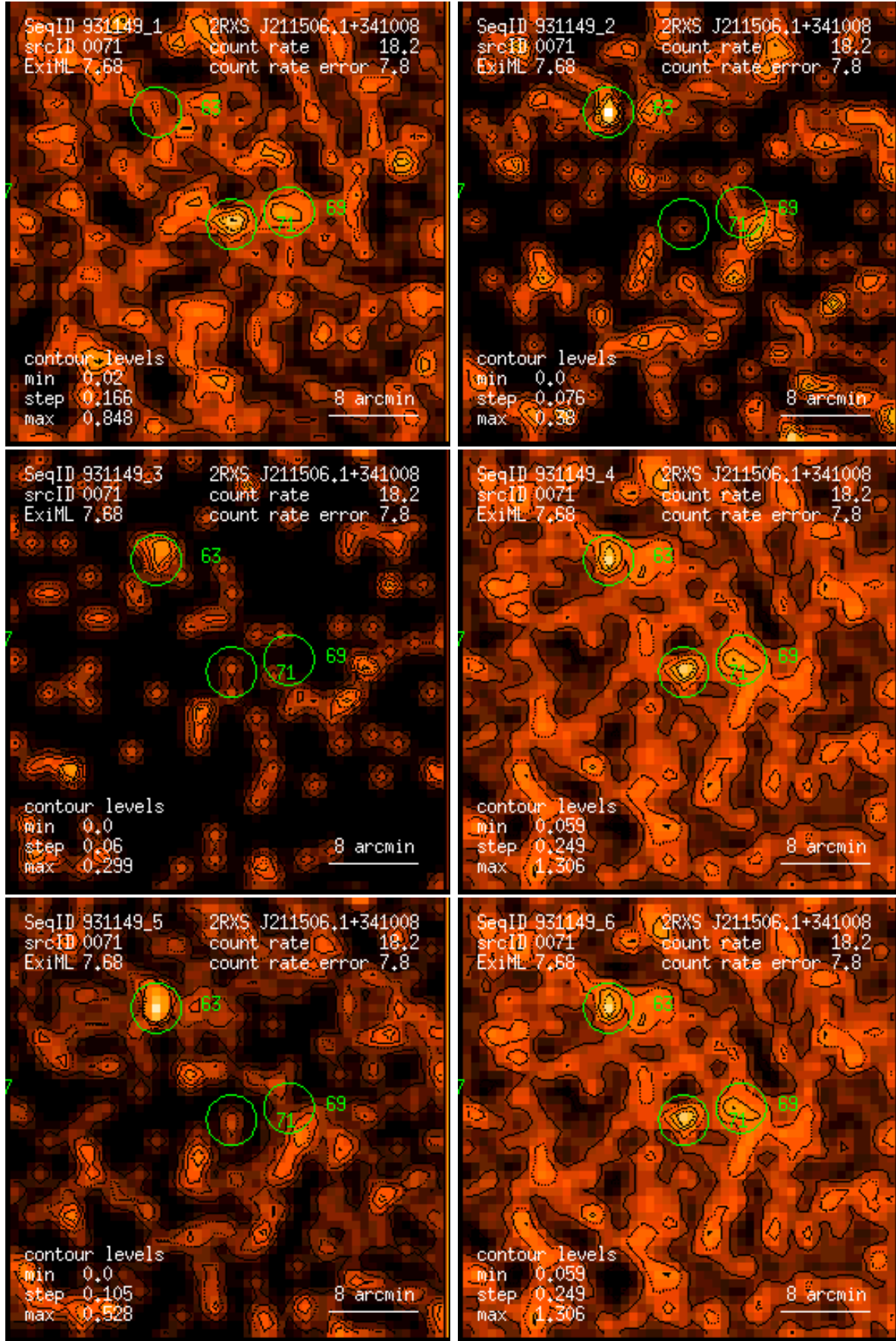
Figure 71: RASS 931149: detection 0071: band rate images, Gaussian filter: (1) PSPC channels 11 – 41, (2) 52 – 90, (3) 91 – 201, (4) 11 – 235, (5) 52 – 201, (6) 11 – 201. Broad band rates in counts/ks. Band rate contour levels in counts/ks/arcmin 2 .
