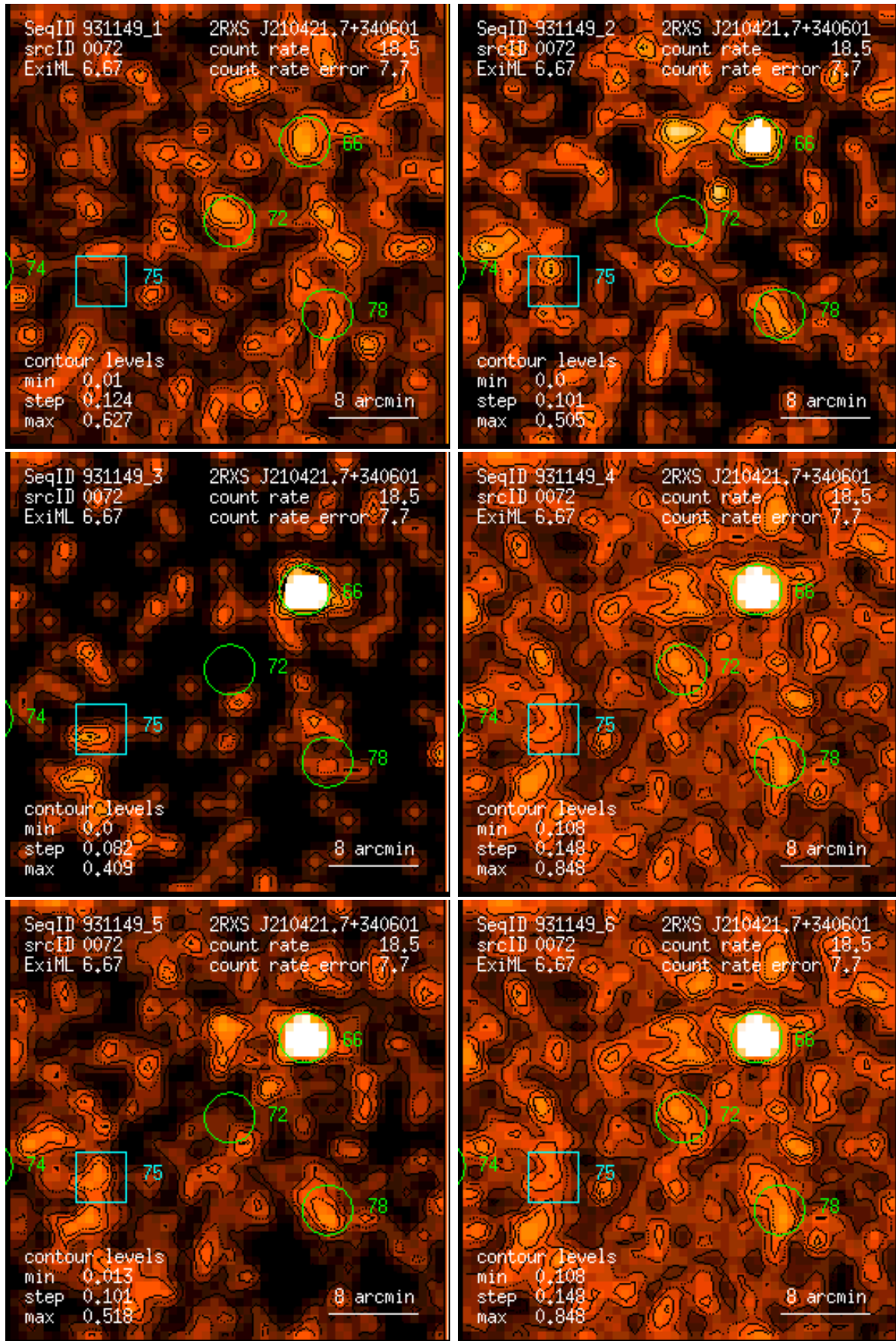
Figure 72: RASS 931149: detection 0072: band rate images, Gaussian filter: (1) PSPC channels 11 – 41, (2) 52 – 90, (3) 91 – 201, (4) 11 – 235, (5) 52 – 201, (6) 11 – 201. Broad band rates in counts/ks. Band rate contour levels in counts/ks/arcmin 2 .
