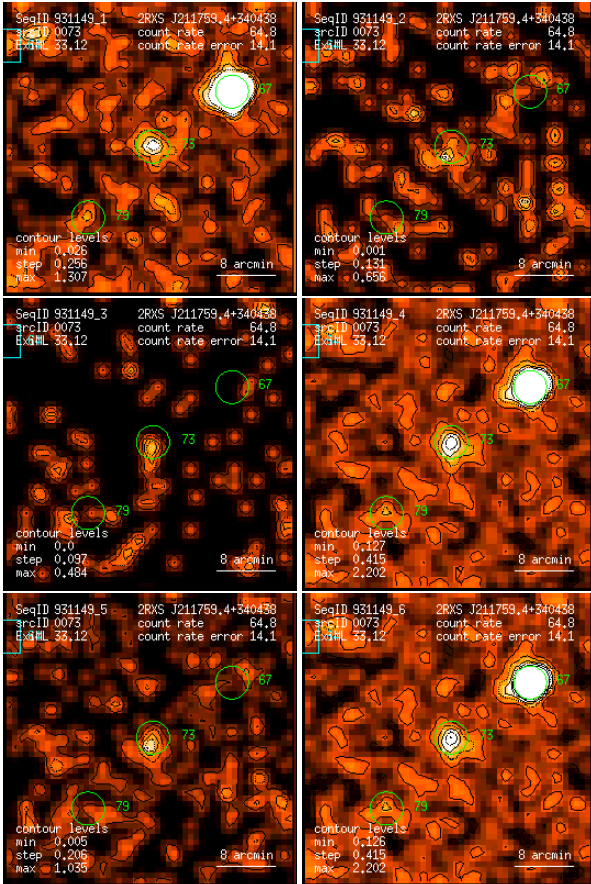
Figure 73: RASS 931149: detection 0073: band rate images, Gaussian filter: (1) PSPC channels 11 – 41, (2) 52 – 90, (3) 91 – 201, (4) 11 – 235, (5) 52 – 201, (6) 11 – 201. Broad band rates in counts/ks. Band rate contour levels in counts/ks/arcmin 2 .
