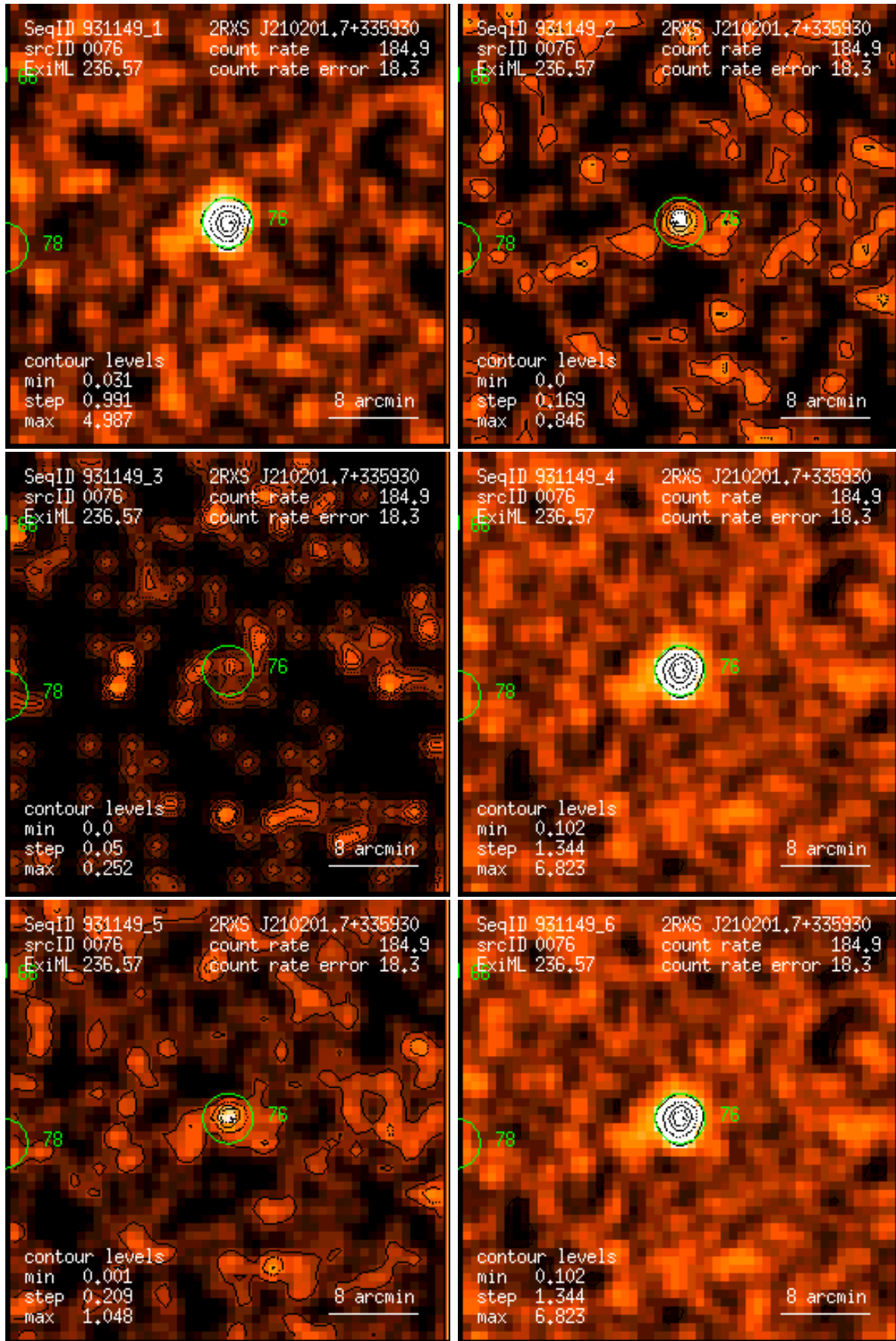
Figure 76: RASS 931149: detection 0076: band rate images, Gaussian filter: (1) PSPC channels 11 – 41, (2) 52 – 90, (3) 91 – 201, (4) 11 – 235, (5) 52 – 201, (6) 11 – 201. Broad band rates in counts/ks. Band rate contour levels in counts/ks/arcmin 2 .
