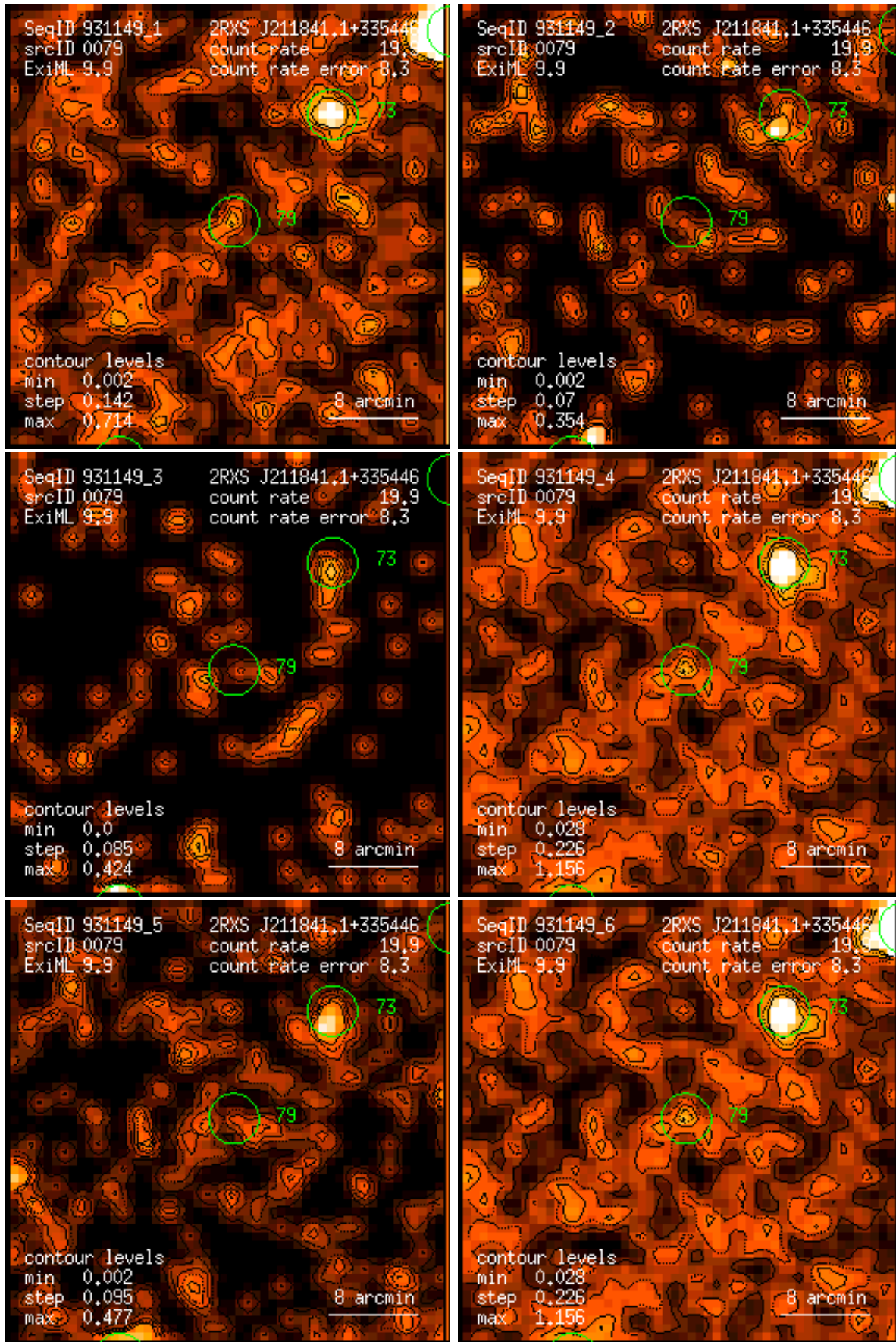
Figure 79: RASS 931149: detection 0079: band rate images, Gaussian filter: (1) PSPC channels 11 – 41, (2) 52 – 90, (3) 91 – 201, (4) 11 – 235, (5) 52 – 201, (6) 11 – 201. Broad band rates in counts/ks. Band rate contour levels in counts/ks/arcmin 2 .
