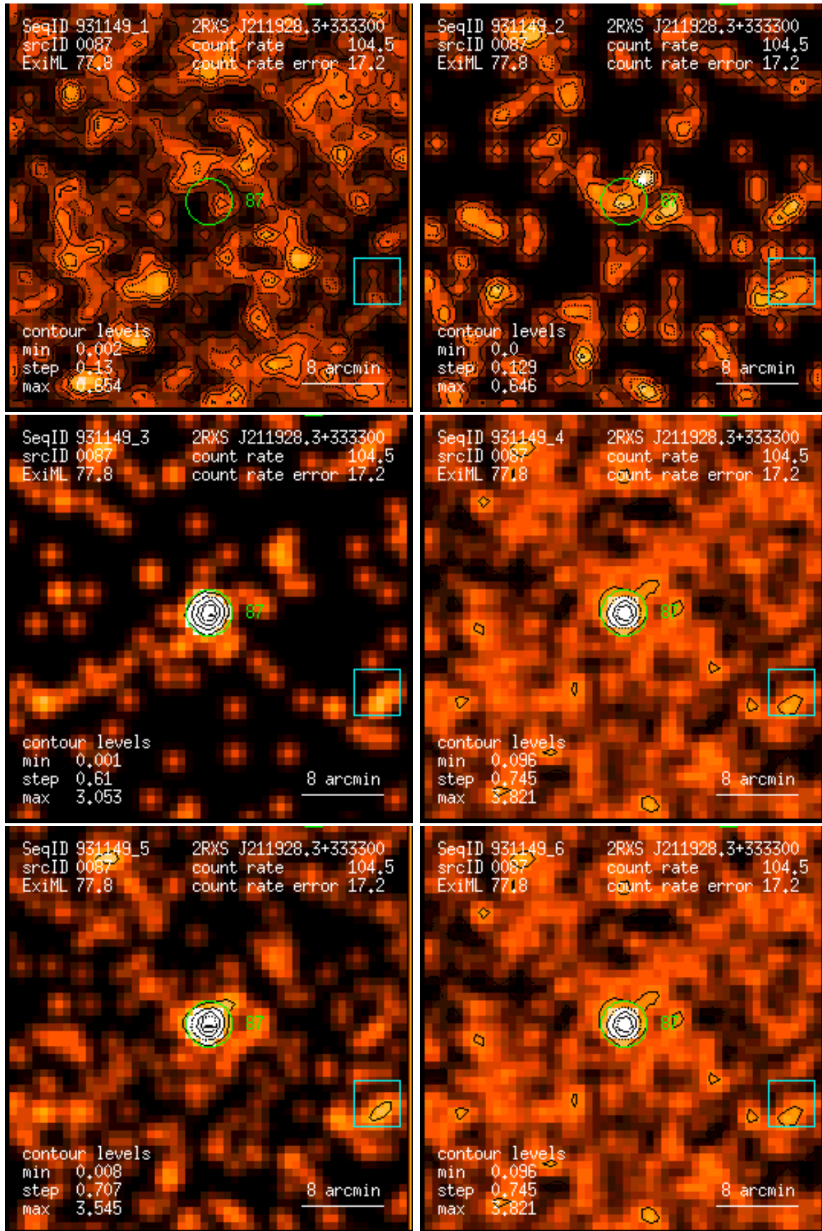
Figure 87: RASS 931149: detection 0087: band rate images, Gaussian filter: (1) PSPC channels 11 – 41, (2) 52 – 90, (3) 91 – 201, (4) 11 – 235, (5) 52 – 201, (6) 11 – 201. Broad band rates in counts/ks. Band rate contour levels in counts/ks/arcmin 2 .
