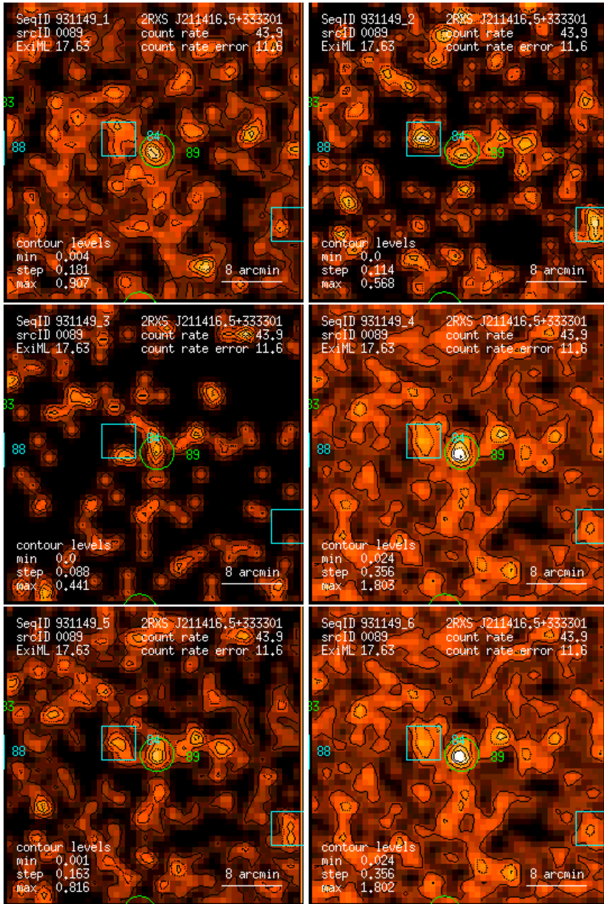
Figure 89: RASS 931149: detection 0089: band rate images, Gaussian filter: (1) PSPC channels 11 – 41, (2) 52 – 90, (3) 91 – 201, (4) 11 – 235, (5) 52 – 201, (6) 11 – 201. Broad band rates in counts/ks. Band rate contour levels in counts/ks/arcmin 2 .
