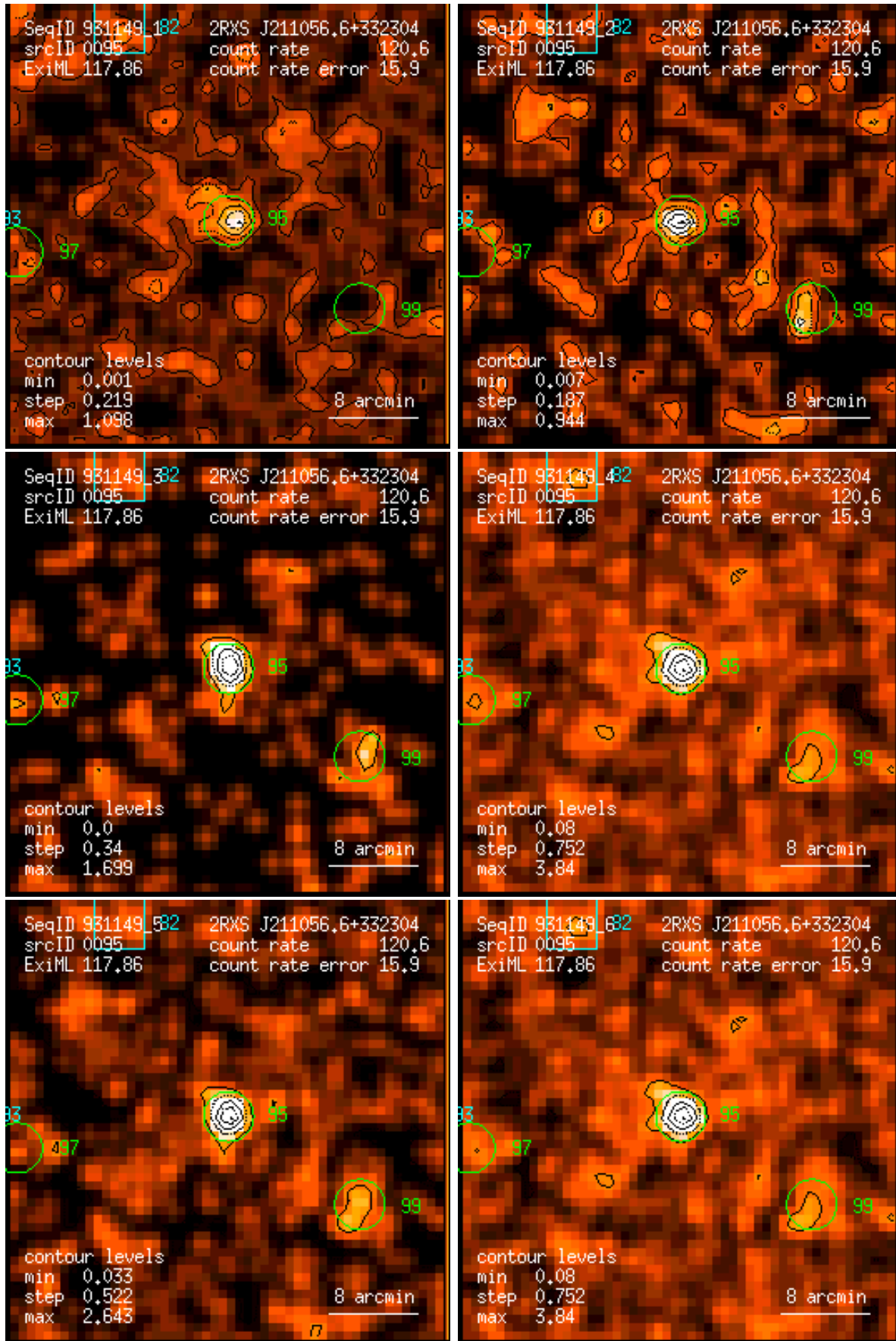
Figure 95: RASS 931149: detection 0095: band rate images, Gaussian filter: (1) PSPC channels 11 – 41, (2) 52 – 90, (3) 91 – 201, (4) 11 – 235, (5) 52 – 201, (6) 11 – 201. Broad band rates in counts/ks. Band rate contour levels in counts/ks/arcmin 2 .
