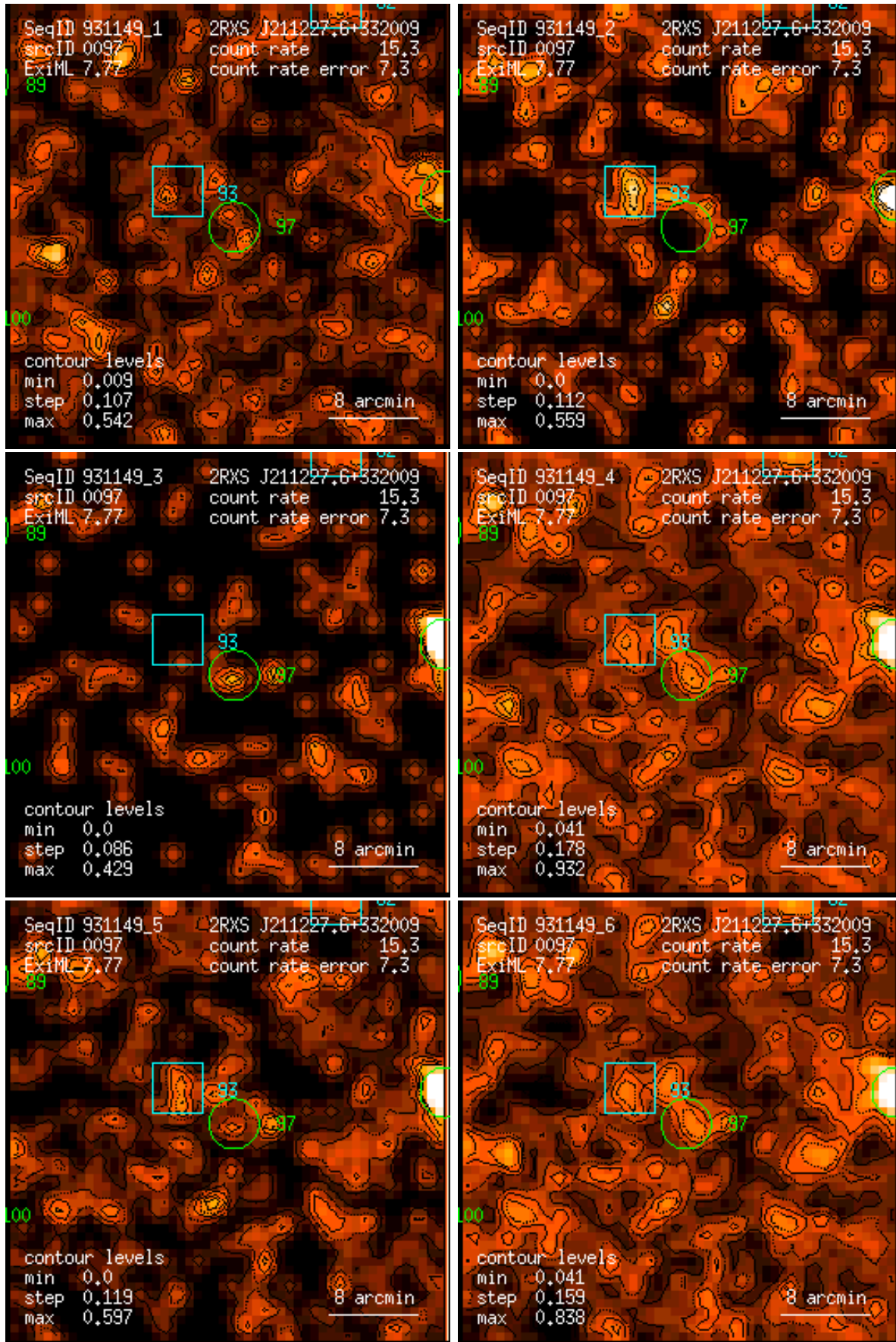
Figure 97: RASS 931149: detection 0097: band rate images, Gaussian filter: (1) PSPC channels 11 – 41, (2) 52 – 90, (3) 91 – 201, (4) 11 – 235, (5) 52 – 201, (6) 11 – 201. Broad band rates in counts/ks. Band rate contour levels in counts/ks/arcmin 2 .
