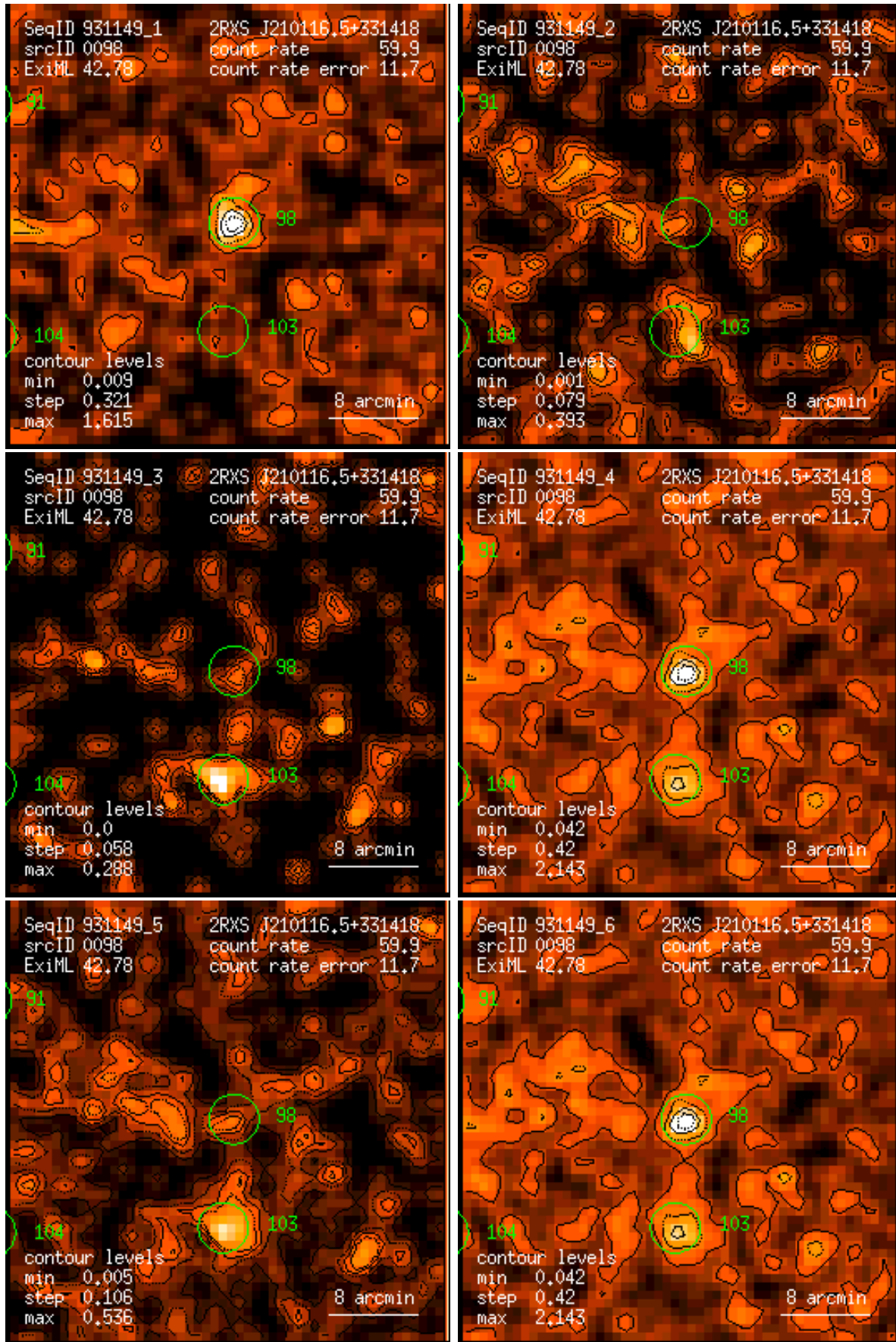
Figure 98: RASS 931149: detection 0098: band rate images, Gaussian filter: (1) PSPC channels 11 – 41, (2) 52 – 90, (3) 91 – 201, (4) 11 – 235, (5) 52 – 201, (6) 11 – 201. Broad band rates in counts/ks. Band rate contour levels in counts/ks/arcmin 2 .
